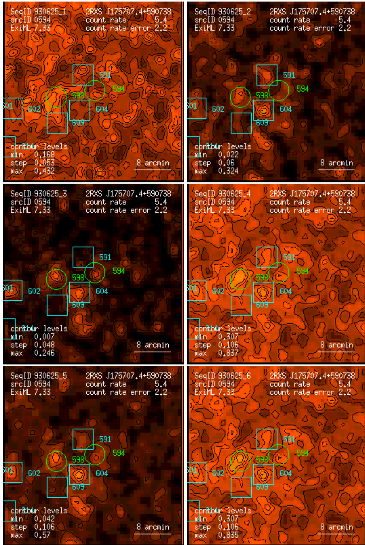
Figure 594: RASS 930625: detection 0594: band rate images, Gaussian filter: (1) PSPC channels 11 – 41, (2) 52 – 90, (3) 91 – 201, (4) 11 – 235, (5) 52 – 201, (6) 11 – 201. Broad band rates in counts/ks. Band rate contour levels in counts/ks/arcmin 2 .
