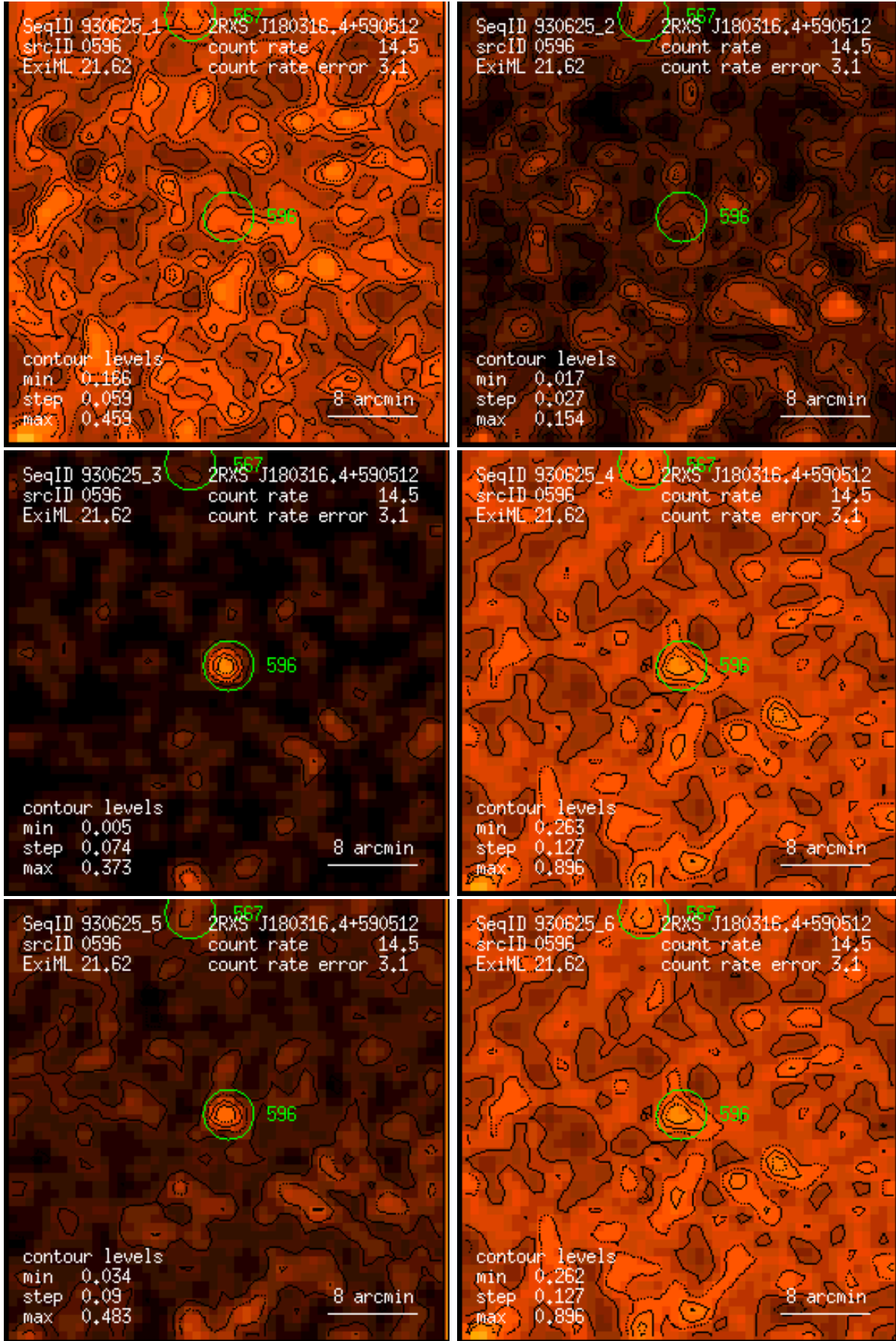
Figure 596: RASS 930625: detection 0596: band rate images, Gaussian filter: (1) PSPC channels 11 – 41, (2) 52 – 90, (3) 91 – 201, (4) 11 – 235, (5) 52 – 201, (6) 11 – 201. Broad band rates in counts/ks. Band rate contour levels in counts/ks/arcmin 2 .
