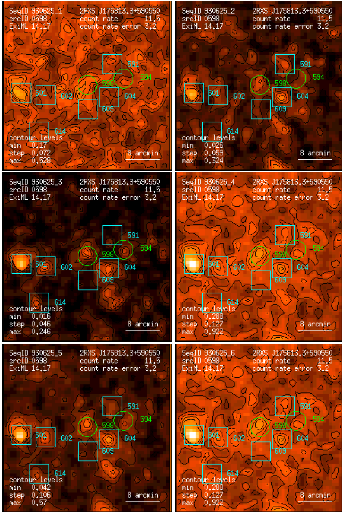
Figure 598: RASS 930625: detection 0598: band rate images, Gaussian filter: (1) PSPC channels 11 – 41, (2) 52 – 90, (3) 91 – 201, (4) 11 – 235, (5) 52 – 201, (6) 11 – 201. Broad band rates in counts/ks. Band rate contour levels in counts/ks/arcmin 2 .
