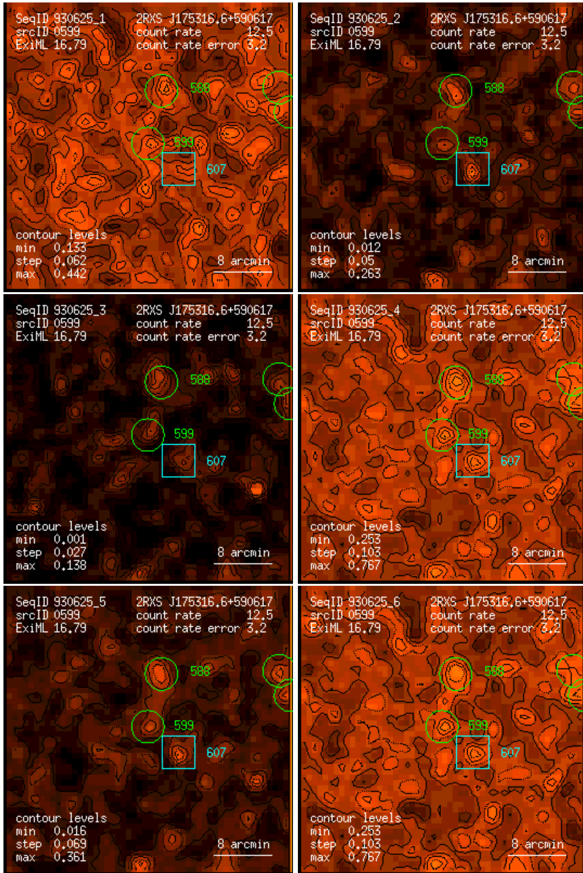
Figure 599: RASS 930625: detection 0599: band rate images, Gaussian filter: (1) PSPC channels 11 – 41, (2) 52 – 90, (3) 91 – 201, (4) 11 – 235, (5) 52 – 201, (6) 11 – 201. Broad band rates in counts/ks. Band rate contour levels in counts/ks/arcmin 2 .
