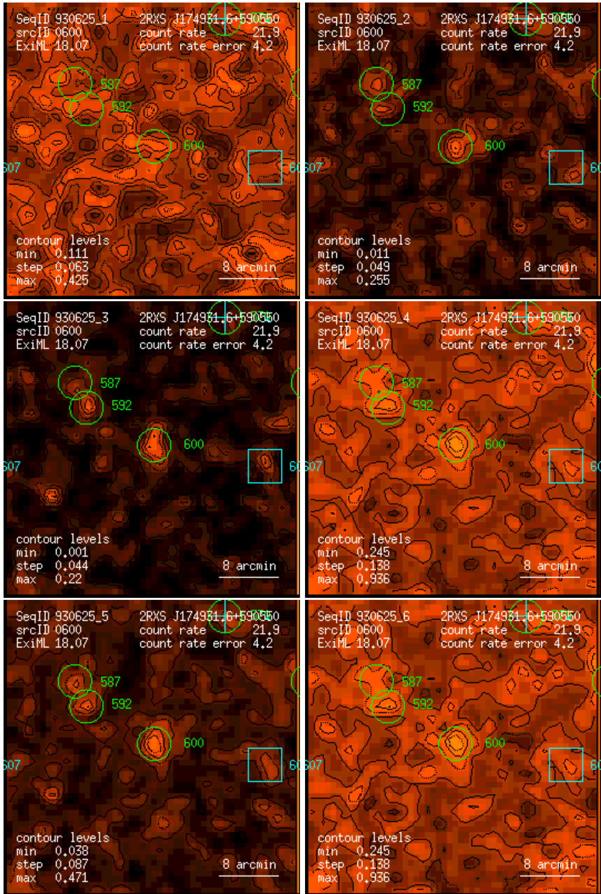
Figure 600: RASS 930625: detection 0600: band rate images, Gaussian filter: (1) PSPC channels 11 – 41, (2) 52 – 90, (3) 91 – 201, (4) 11 – 235, (5) 52 – 201, (6) 11 – 201. Broad band rates in counts/ks. Band rate contour levels in counts/ks/arcmin 2 .
