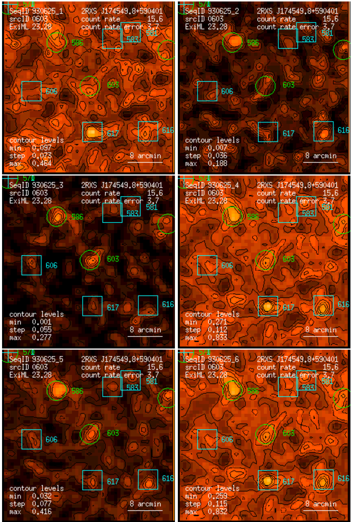
Figure 603: RASS 930625: detection 0603: band rate images, Gaussian filter: (1) PSPC channels 11 – 41, (2) 52 – 90, (3) 91 – 201, (4) 11 – 235, (5) 52 – 201, (6) 11 – 201. Broad band rates in counts/ks. Band rate contour levels in counts/ks/arcmin 2 .
