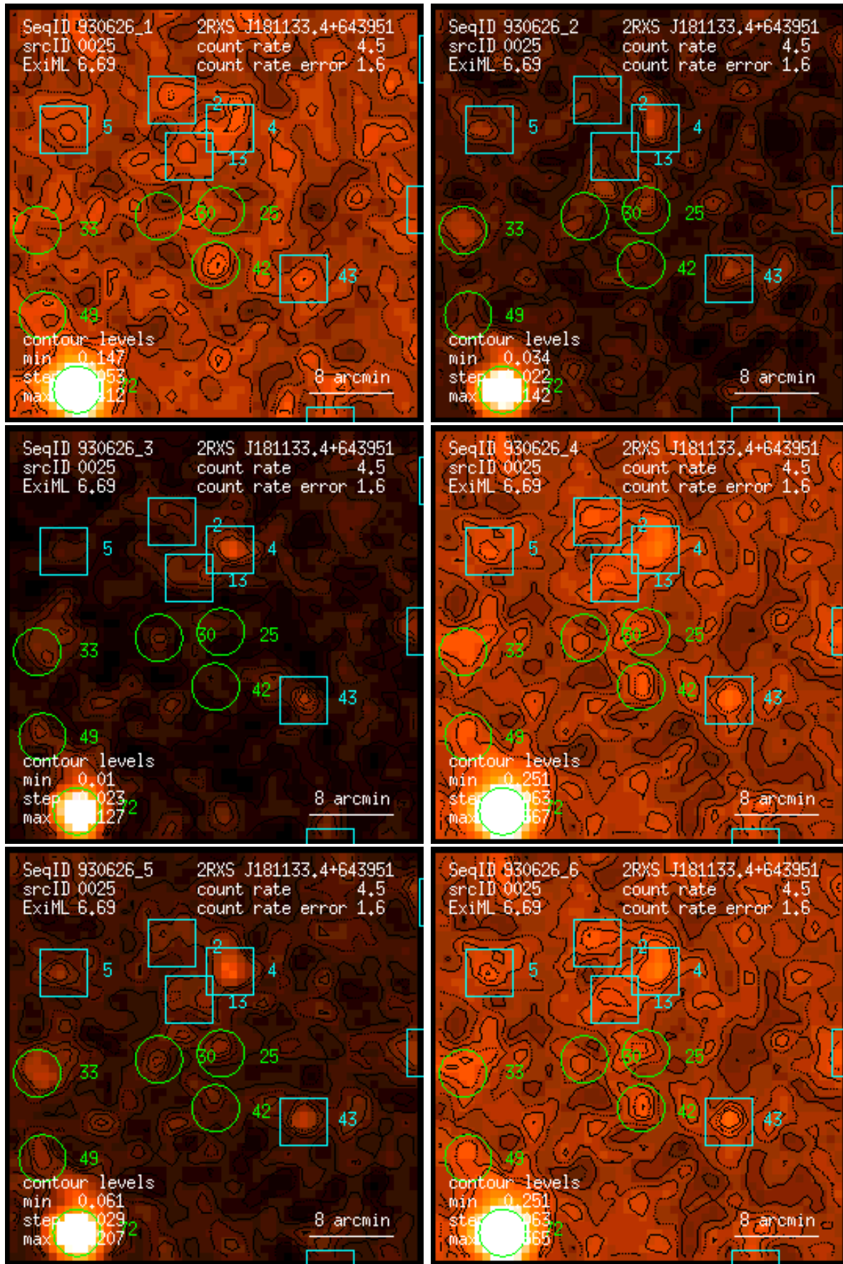
Figure 25: RASS 930626: detection 0025: band rate images, Gaussian filter: (1) PSPC channels 11 – 41, (2) 52 – 90, (3) 91 – 201, (4) 11 – 235, (5) 52 – 201, (6) 11 – 201. Broad band rates in counts/ks. Band rate contour levels in counts/ks/arcmin 2 .
