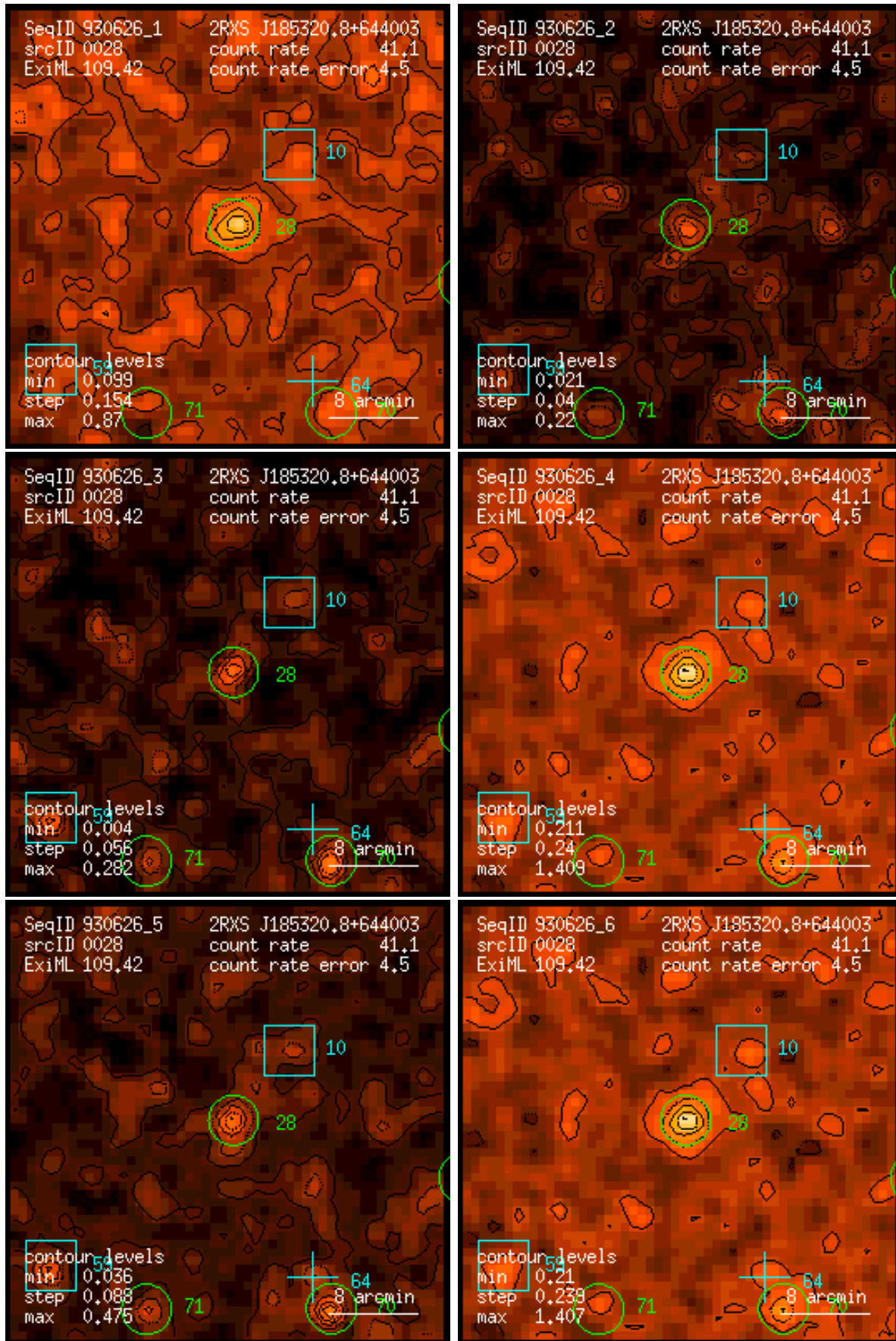
Figure 28: RASS 930626: detection 0028: band rate images, Gaussian filter: (1) PSPC channels 11 – 41, (2) 52 – 90, (3) 91 – 201, (4) 11 – 235, (5) 52 – 201, (6) 11 – 201. Broad band rates in counts/ks. Band rate contour levels in counts/ks/arcmin 2 .
