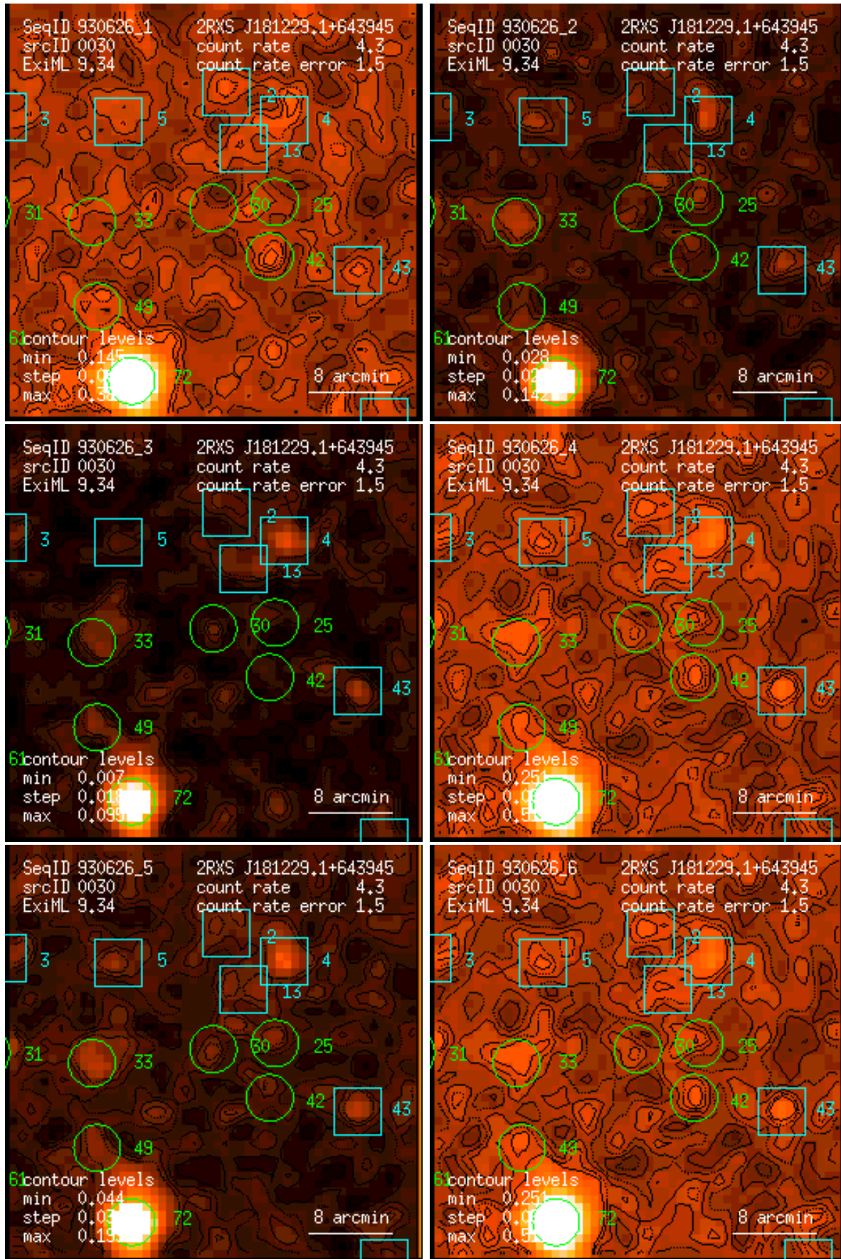
Figure 30: RASS 930626: detection 0030: band rate images, Gaussian filter: (1) PSPC channels 11 – 41, (2) 52 – 90, (3) 91 – 201, (4) 11 – 235, (5) 52 – 201, (6) 11 – 201. Broad band rates in counts/ks. Band rate contour levels in counts/ks/arcmin 2 .
