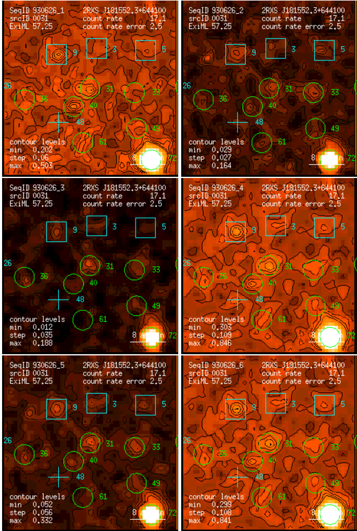
Figure 31: RASS 930626: detection 0031: band rate images, Gaussian filter: (1) PSPC channels 11 – 41, (2) 52 – 90, (3) 91 – 201, (4) 11 – 235, (5) 52 – 201, (6) 11 – 201. Broad band rates in counts/ks. Band rate contour levels in counts/ks/arcmin 2 .
