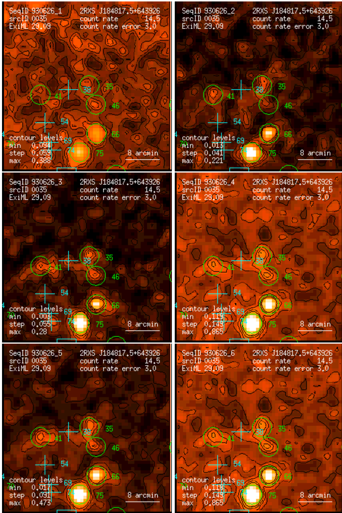
Figure 35: RASS 930626: detection 0035: band rate images, Gaussian filter: (1) PSPC channels 11 – 41, (2) 52 – 90, (3) 91 – 201, (4) 11 – 235, (5) 52 – 201, (6) 11 – 201. Broad band rates in counts/ks. Band rate contour levels in counts/ks/arcmin 2 .
