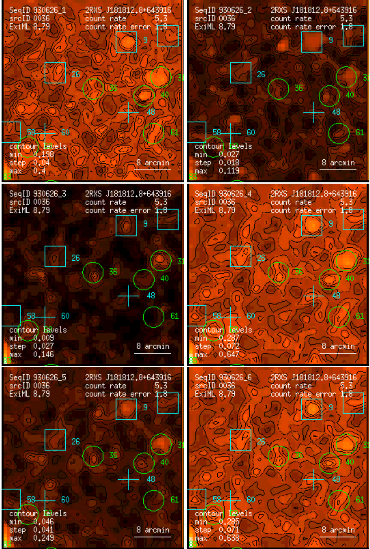
Figure 36: RASS 930626: detection 0036: band rate images, Gaussian filter: (1) PSPC channels 11 – 41, (2) 52 – 90, (3) 91 – 201, (4) 11 – 235, (5) 52 – 201, (6) 11 – 201. Broad band rates in counts/ks. Band rate contour levels in counts/ks/arcmin 2 .
