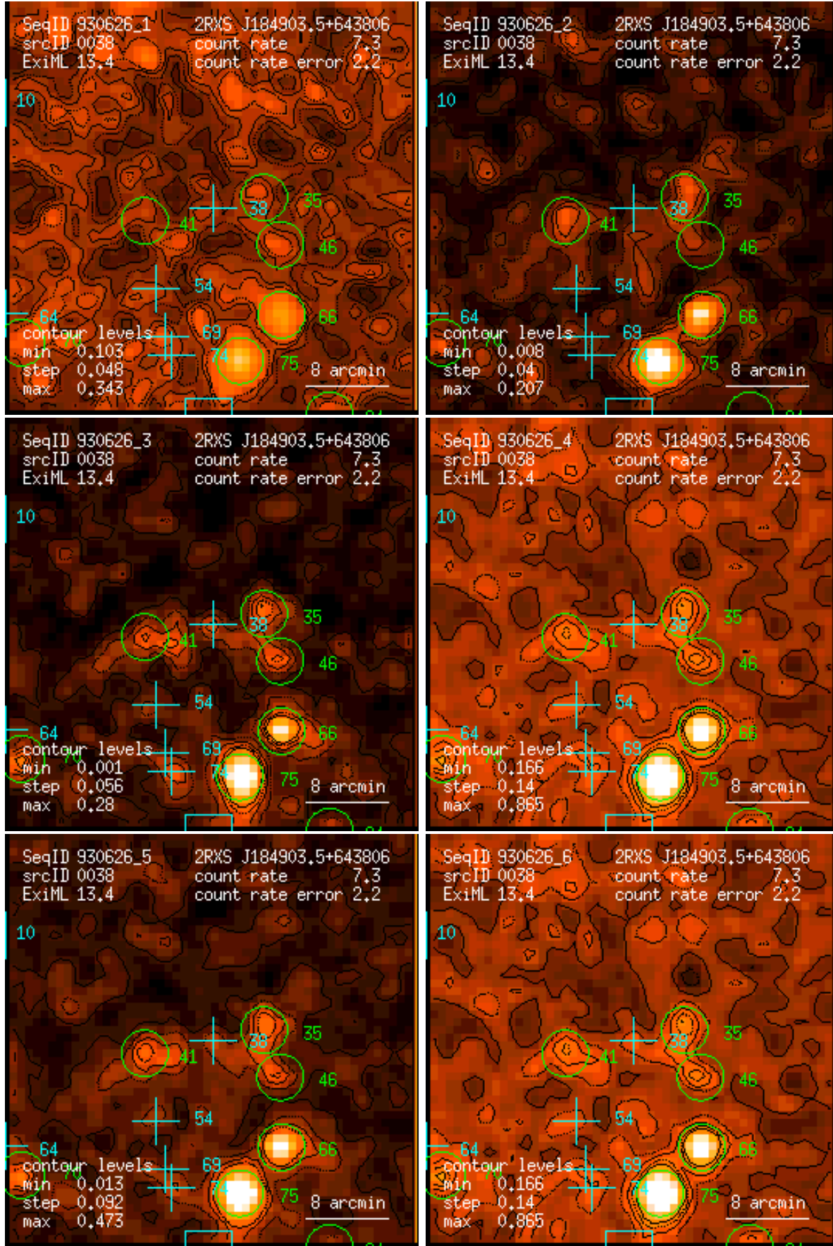
Figure 38: RASS 930626: detection 0038: band rate images, Gaussian filter: (1) PSPC channels 11 – 41, (2) 52 – 90, (3) 91 – 201, (4) 11 – 235, (5) 52 – 201, (6) 11 – 201. Broad band rates in counts/ks. Band rate contour levels in counts/ks/arcmin 2 .
