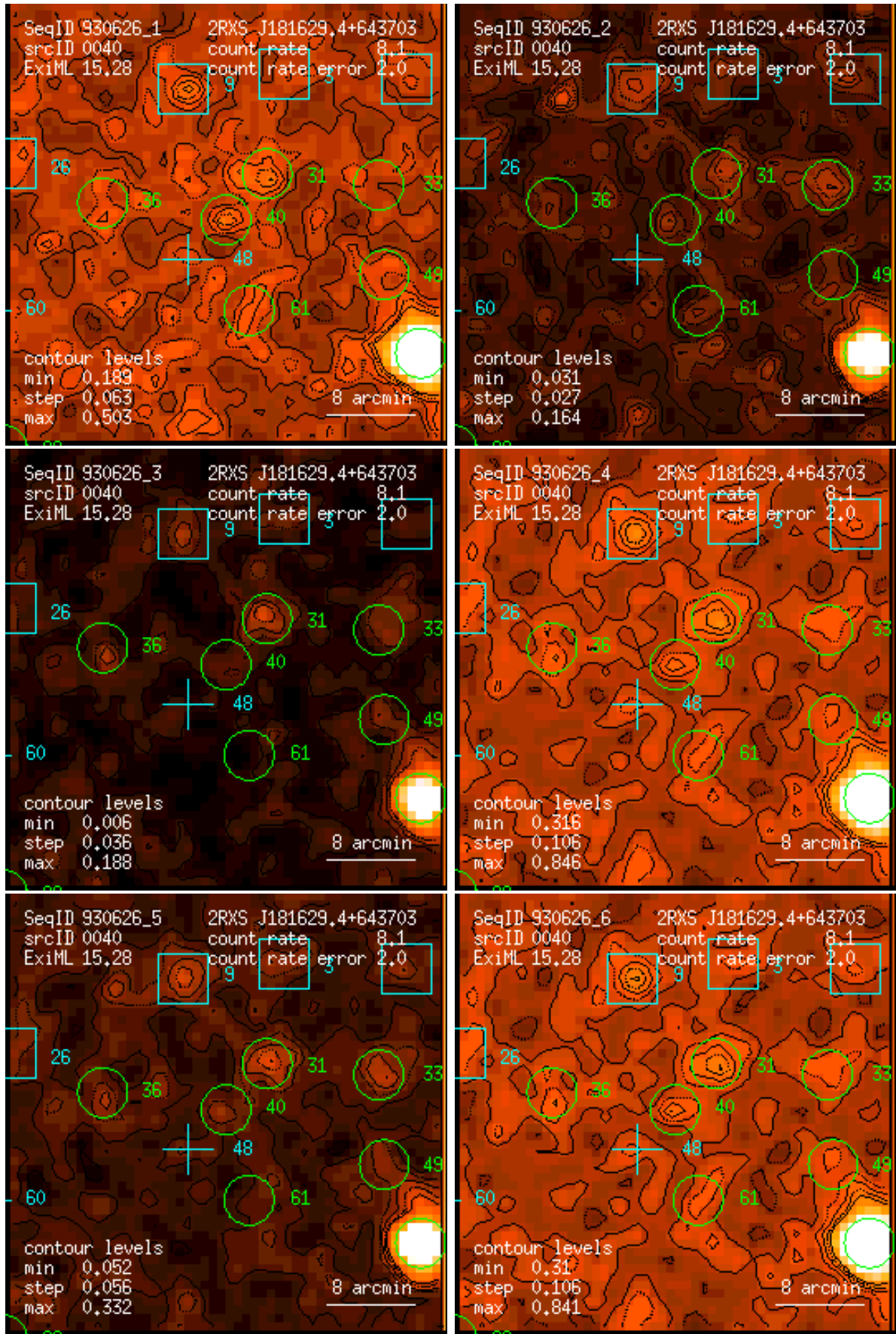
Figure 40: RASS 930626: detection 0040: band rate images, Gaussian filter: (1) PSPC channels 11 – 41, (2) 52 – 90, (3) 91 – 201, (4) 11 – 235, (5) 52 – 201, (6) 11 – 201. Broad band rates in counts/ks. Band rate contour levels in counts/ks/arcmin 2 .
