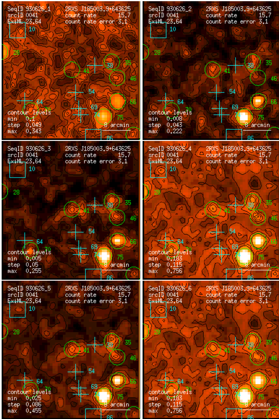
Figure 41: RASS 930626: detection 0041: band rate images, Gaussian filter: (1) PSPC channels 11 – 41, (2) 52 – 90, (3) 91 – 201, (4) 11 – 235, (5) 52 – 201, (6) 11 – 201. Broad band rates in counts/ks. Band rate contour levels in counts/ks/arcmin 2 .
