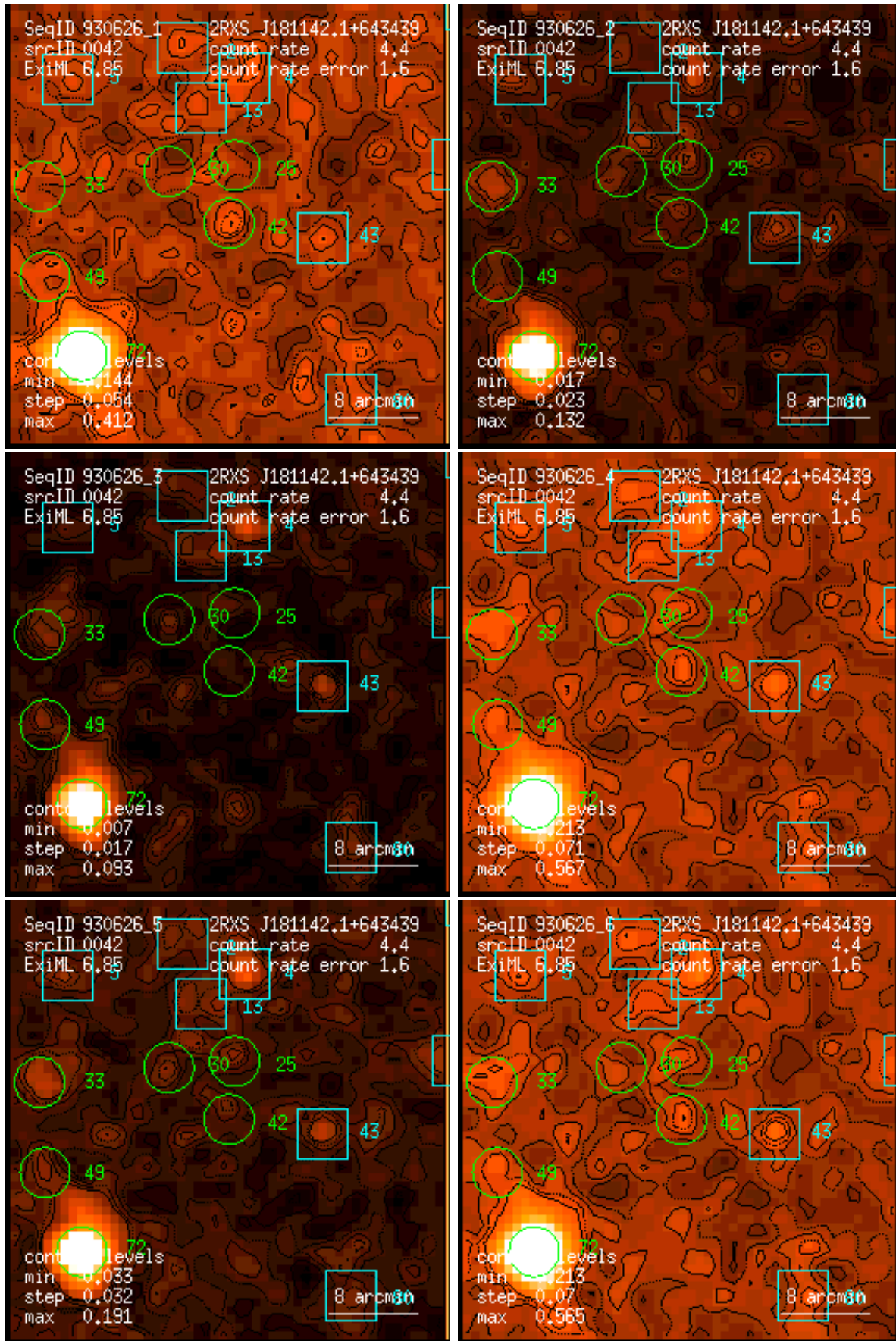
Figure 42: RASS 930626: detection 0042: band rate images, Gaussian filter: (1) PSPC channels 11 – 41, (2) 52 – 90, (3) 91 – 201, (4) 11 – 235, (5) 52 – 201, (6) 11 – 201. Broad band rates in counts/ks. Band rate contour levels in counts/ks/arcmin 2 .
