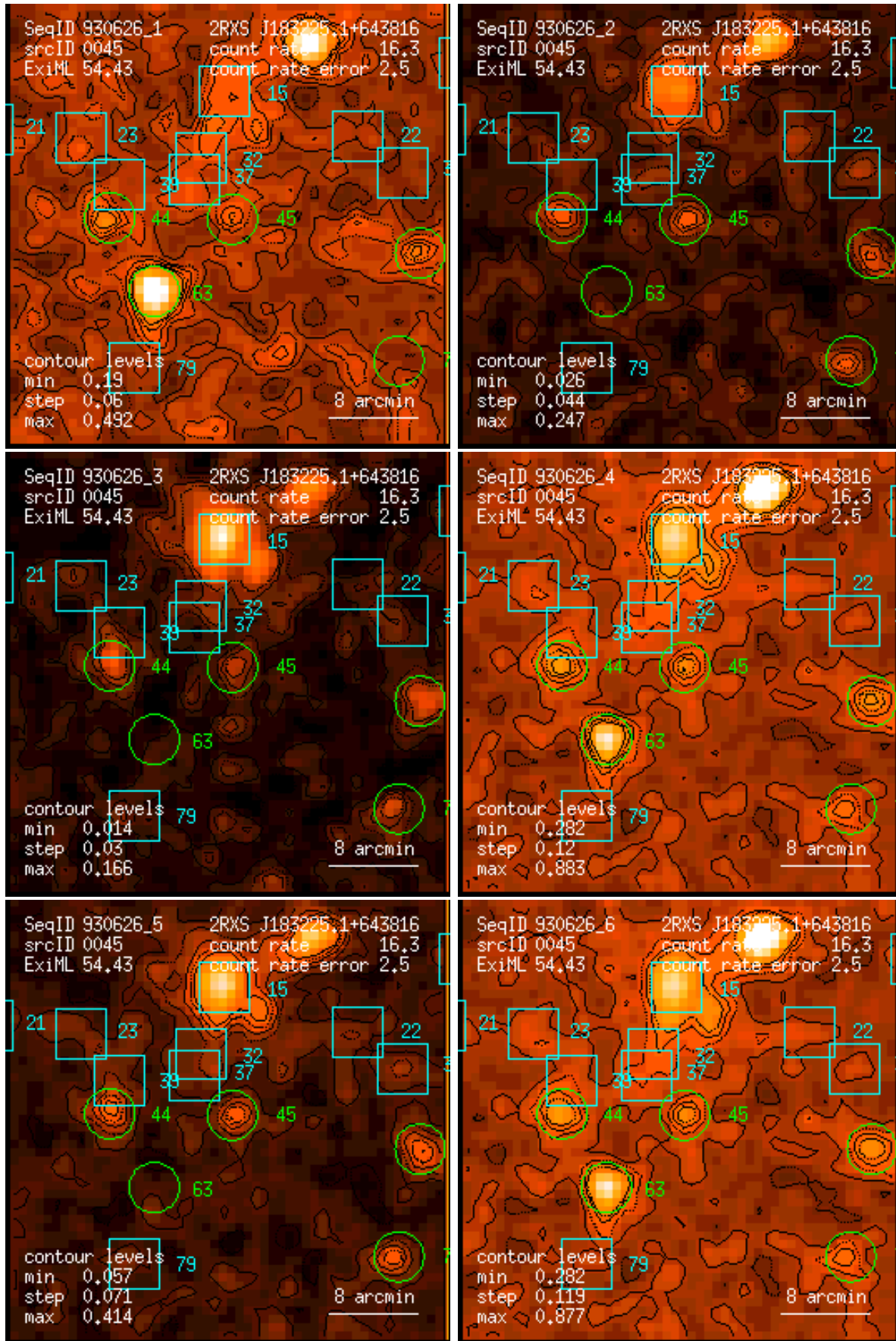
Figure 45: RASS 930626: detection 0045: band rate images, Gaussian filter: (1) PSPC channels 11 – 41, (2) 52 – 90, (3) 91 – 201, (4) 11 – 235, (5) 52 – 201, (6) 11 – 201. Broad band rates in counts/ks. Band rate contour levels in counts/ks/arcmin 2 .
