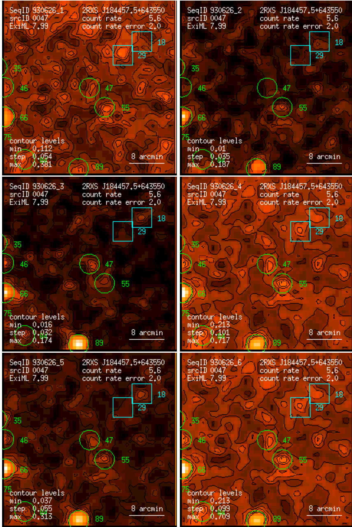
Figure 47: RASS 930626: detection 0047: band rate images, Gaussian filter: (1) PSPC channels 11 – 41, (2) 52 – 90, (3) 91 – 201, (4) 11 – 235, (5) 52 – 201, (6) 11 – 201. Broad band rates in counts/ks. Band rate contour levels in counts/ks/arcmin 2 .
