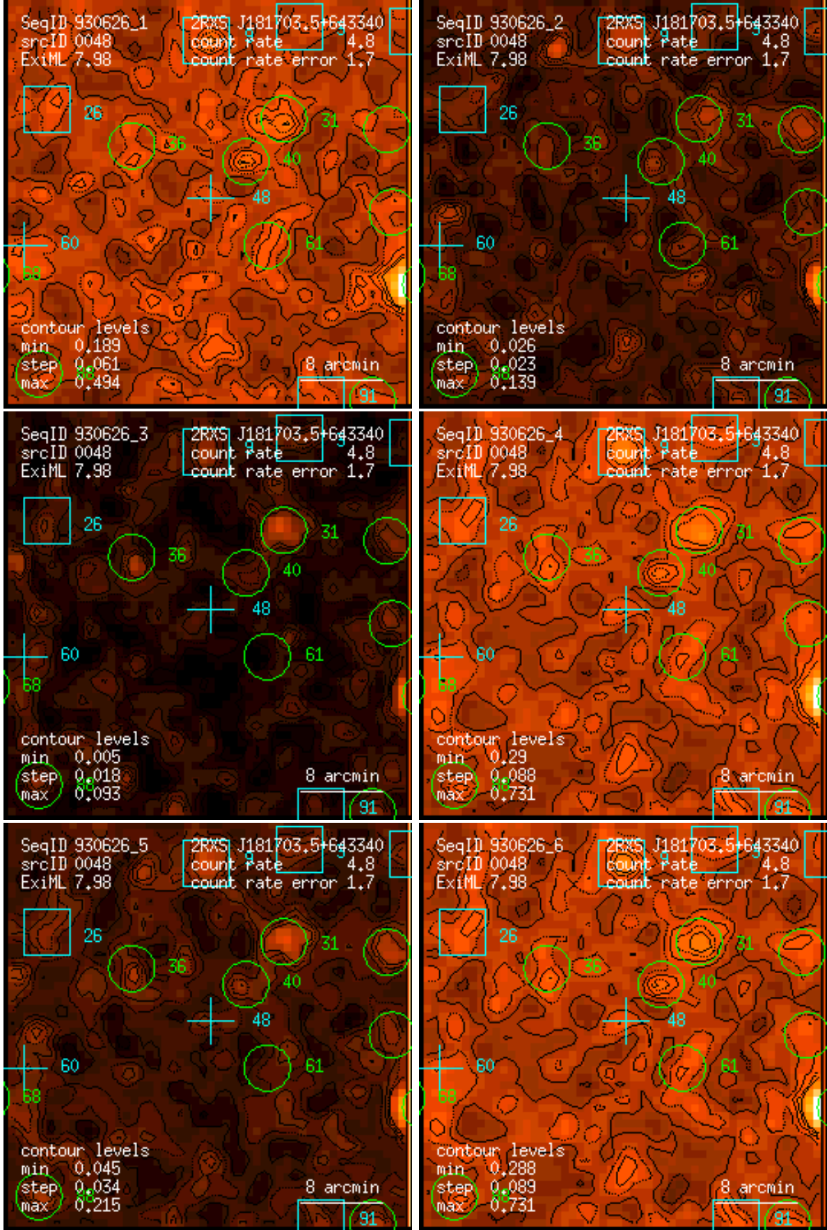
Figure 48: RASS 930626: detection 0048: band rate images, Gaussian filter: (1) PSPC channels 11 – 41, (2) 52 – 90, (3) 91 – 201, (4) 11 – 235, (5) 52 – 201, (6) 11 – 201. Broad band rates in counts/ks. Band rate contour levels in counts/ks/arcmin 2 .
