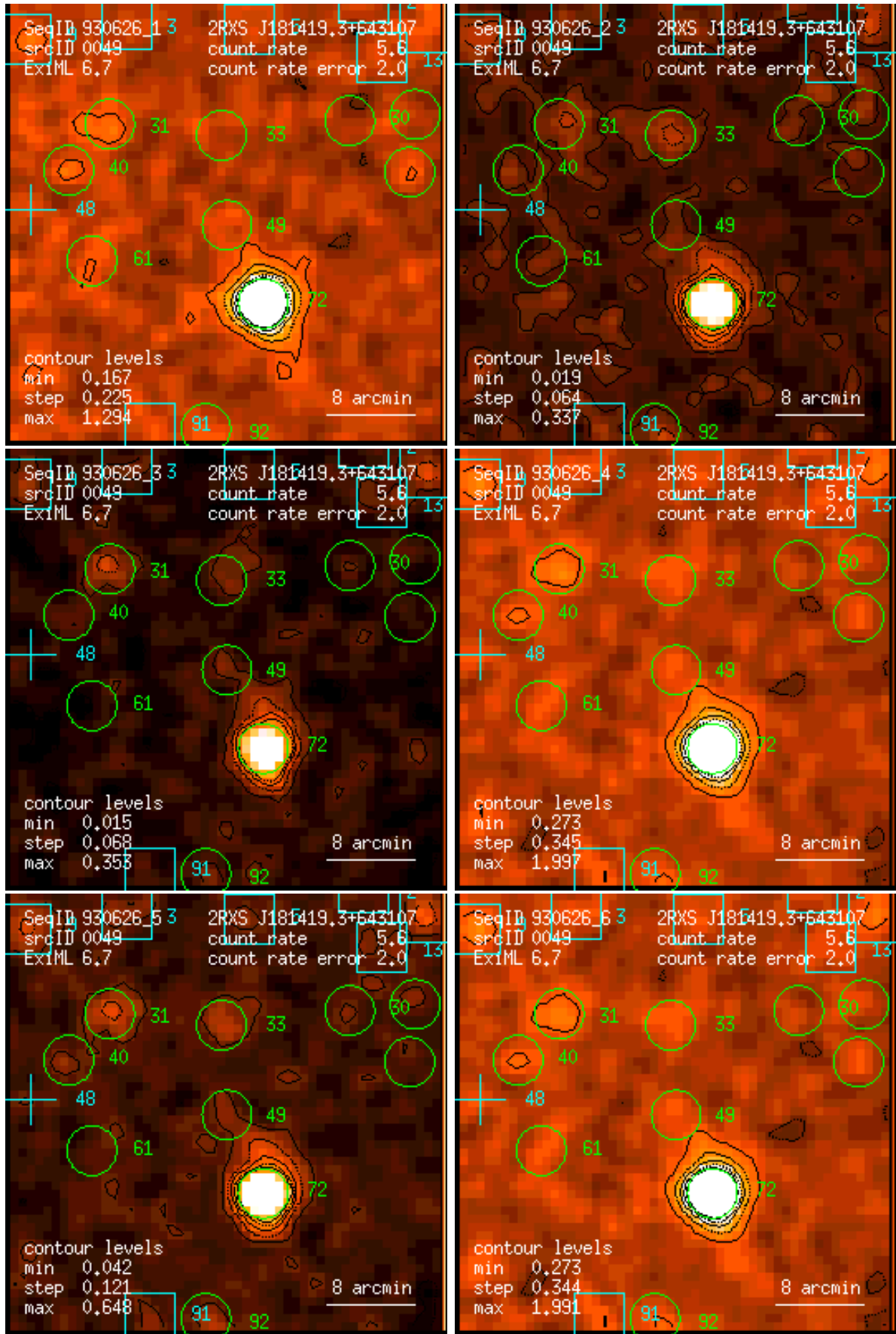
Figure 49: RASS 930626: detection 0049: band rate images, Gaussian filter: (1) PSPC channels 11 – 41, (2) 52 – 90, (3) 91 – 201, (4) 11 – 235, (5) 52 – 201, (6) 11 – 201. Broad band rates in counts/ks. Band rate contour levels in counts/ks/arcmin 2 .
