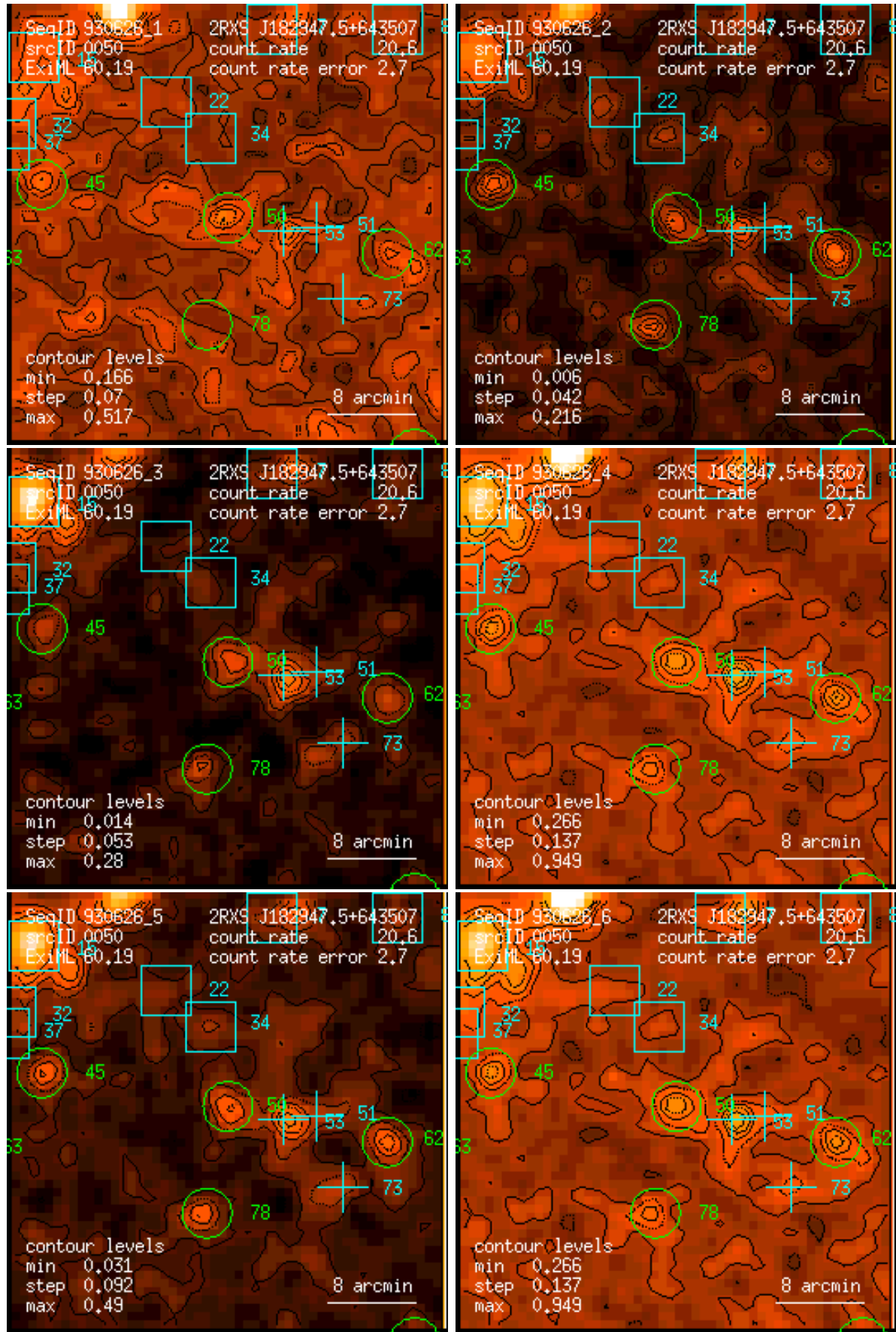
Figure 50: RASS 930626: detection 0050: band rate images, Gaussian filter: (1) PSPC channels 11 – 41, (2) 52 – 90, (3) 91 – 201, (4) 11 – 235, (5) 52 – 201, (6) 11 – 201. Broad band rates in counts/ks. Band rate contour levels in counts/ks/arcmin 2 .
