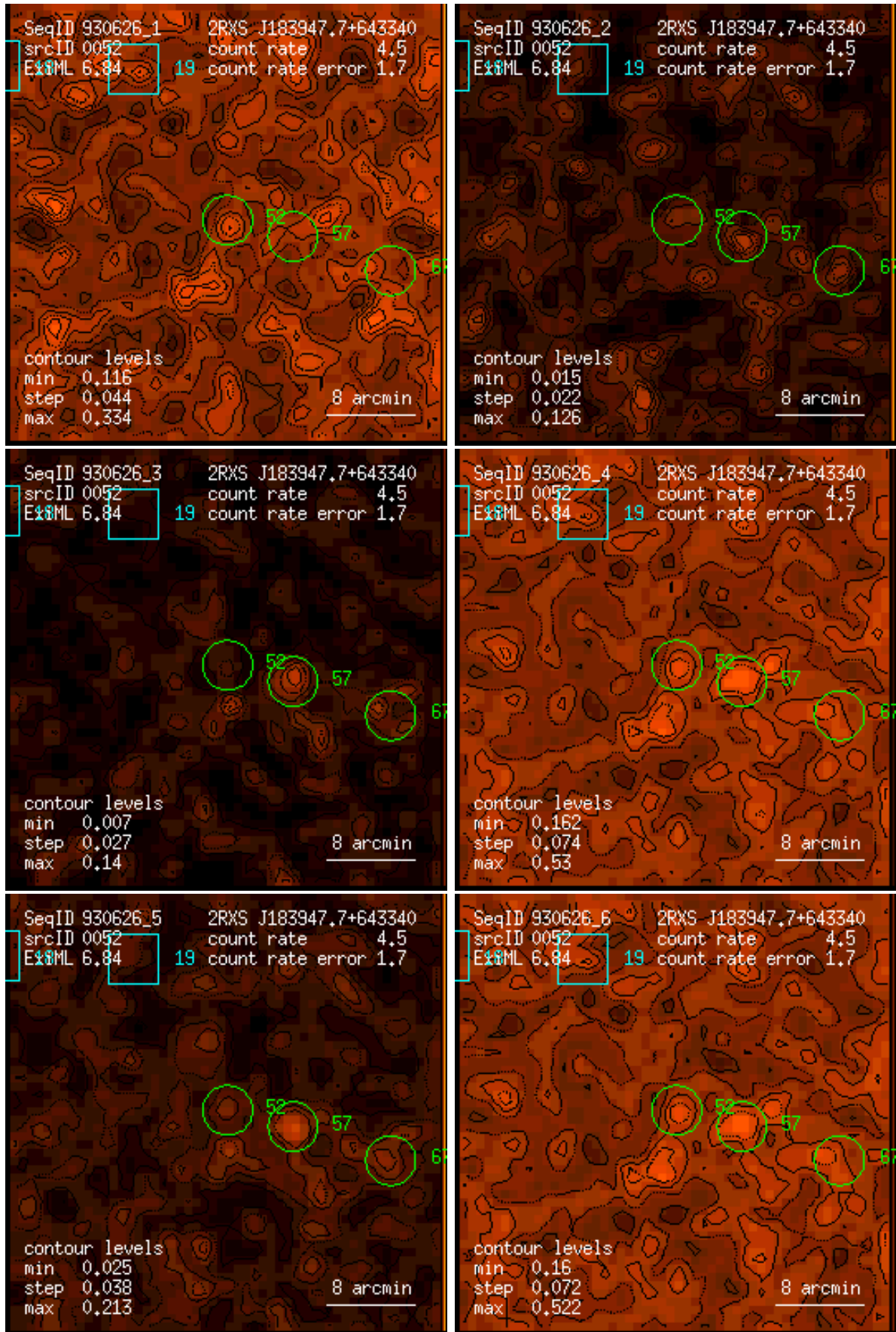
Figure 52: RASS 930626: detection 0052: band rate images, Gaussian filter: (1) PSPC channels 11 – 41, (2) 52 – 90, (3) 91 – 201, (4) 11 – 235, (5) 52 – 201, (6) 11 – 201. Broad band rates in counts/ks. Band rate contour levels in counts/ks/arcmin 2 .
