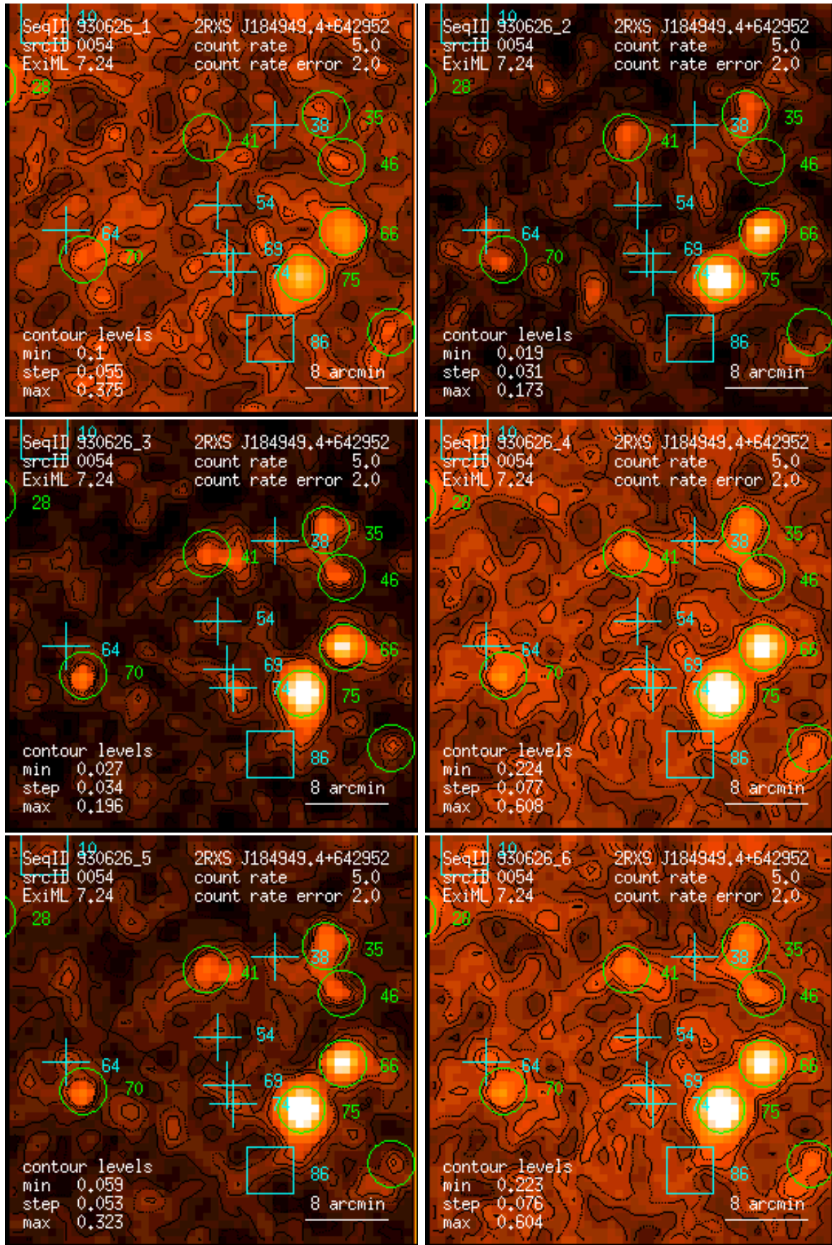
Figure 54: RASS 930626: detection 0054: band rate images, Gaussian filter: (1) PSPC channels 11 – 41, (2) 52 – 90, (3) 91 – 201, (4) 11 – 235, (5) 52 – 201, (6) 11 – 201. Broad band rates in counts/ks. Band rate contour levels in counts/ks/arcmin 2 .
