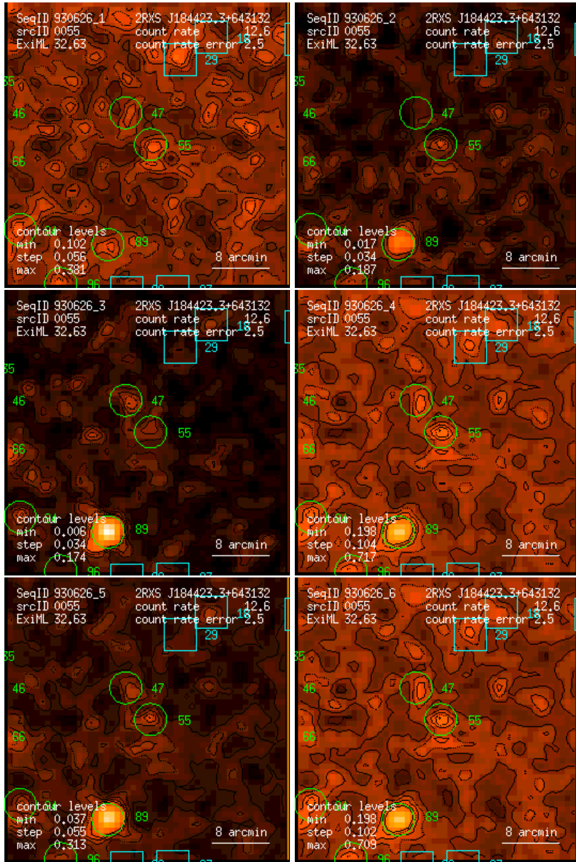
Figure 55: RASS 930626: detection 0055: band rate images, Gaussian filter: (1) PSPC channels 11 – 41, (2) 52 – 90, (3) 91 – 201, (4) 11 – 235, (5) 52 – 201, (6) 11 – 201. Broad band rates in counts/ks. Band rate contour levels in counts/ks/arcmin 2 .
