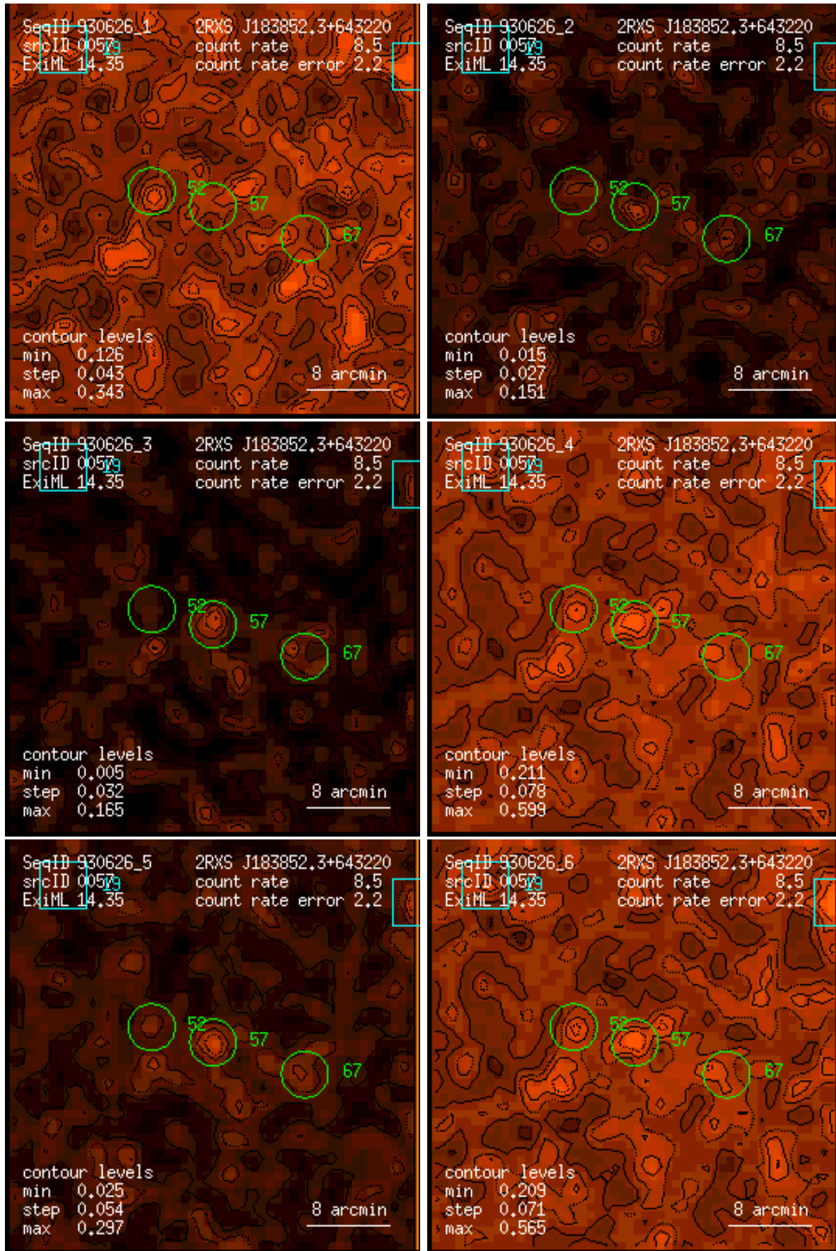
Figure 57: RASS 930626: detection 0057: band rate images, Gaussian filter: (1) PSPC channels 11 – 41, (2) 52 – 90, (3) 91 – 201, (4) 11 – 235, (5) 52 – 201, (6) 11 – 201. Broad band rates in counts/ks. Band rate contour levels in counts/ks/arcmin 2 .
