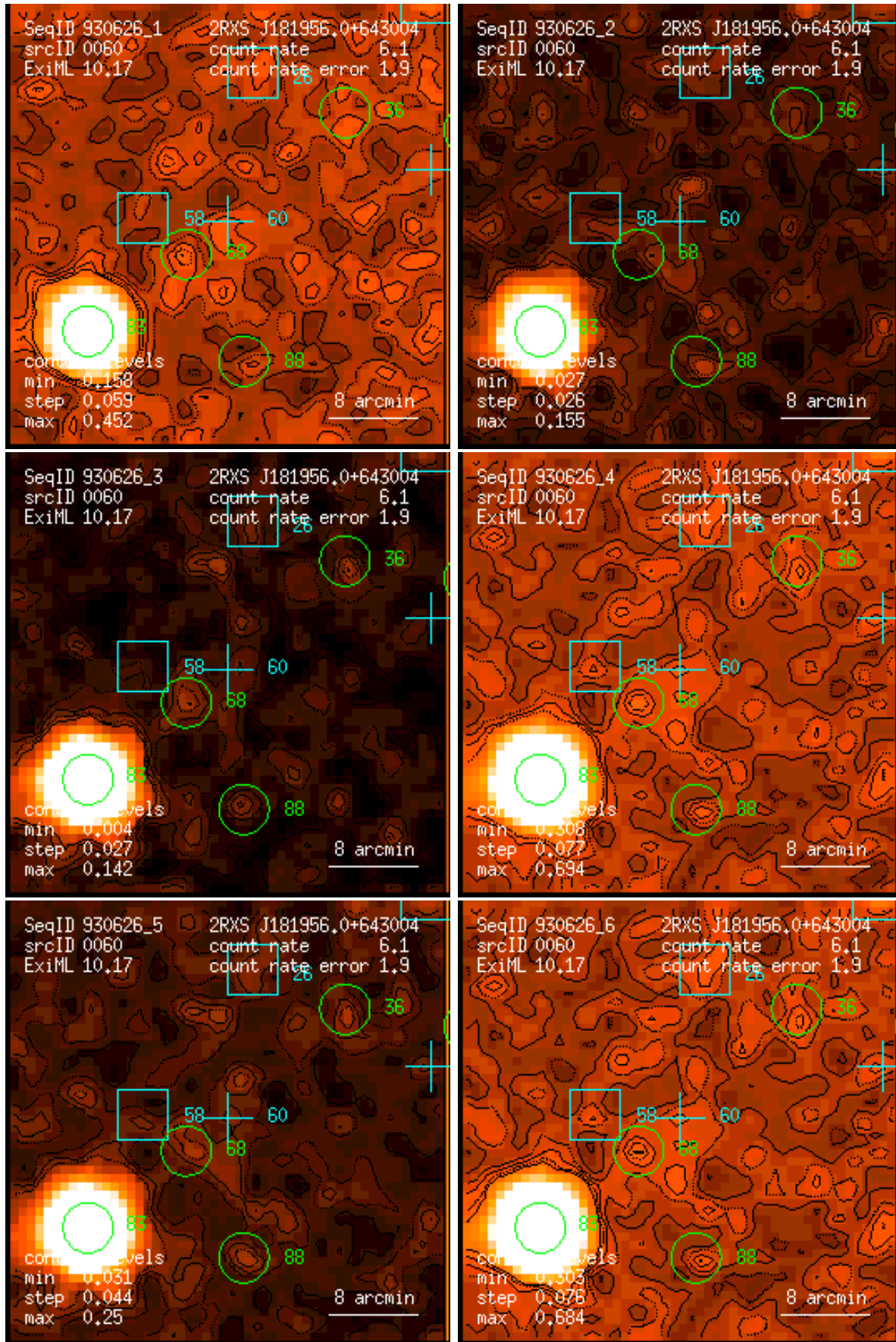
Figure 60: RASS 930626: detection 0060: band rate images, Gaussian filter: (1) PSPC channels 11 – 41, (2) 52 – 90, (3) 91 – 201, (4) 11 – 235, (5) 52 – 201, (6) 11 – 201. Broad band rates in counts/ks. Band rate contour levels in counts/ks/arcmin 2 .
