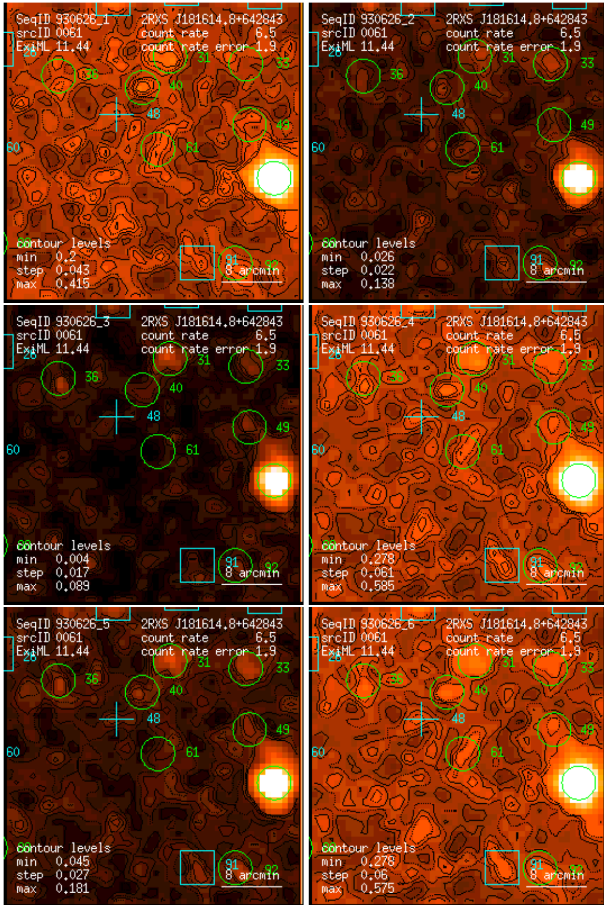
Figure 61: RASS 930626: detection 0061: band rate images, Gaussian filter: (1) PSPC channels 11 – 41, (2) 52 – 90, (3) 91 – 201, (4) 11 – 235, (5) 52 – 201, (6) 11 – 201. Broad band rates in counts/ks. Band rate contour levels in counts/ks/arcmin 2 .
