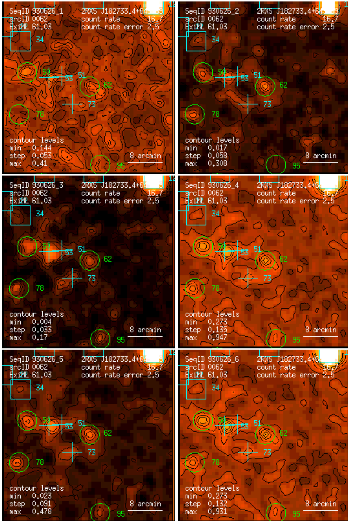
Figure 62: RASS 930626: detection 0062: band rate images, Gaussian filter: (1) PSPC channels 11 – 41, (2) 52 – 90, (3) 91 – 201, (4) 11 – 235, (5) 52 – 201, (6) 11 – 201. Broad band rates in counts/ks. Band rate contour levels in counts/ks/arcmin 2 .
