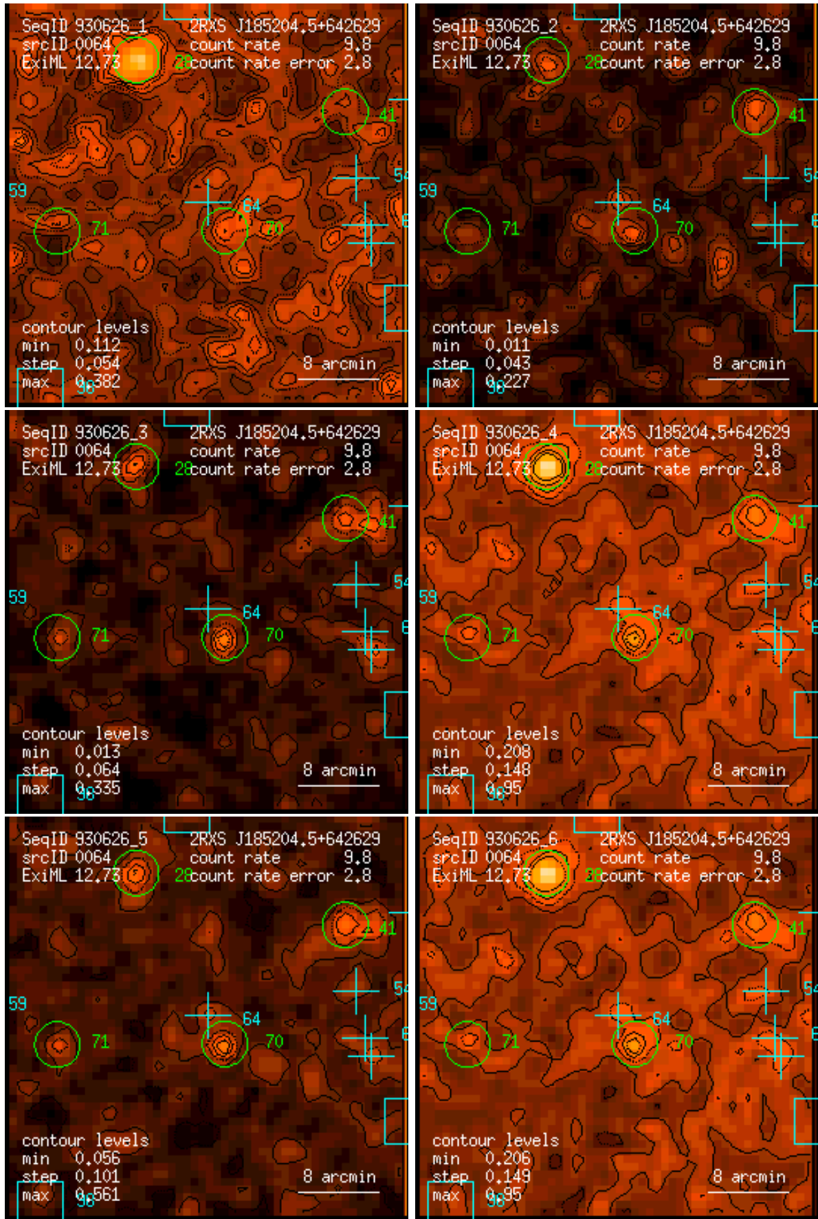
Figure 64: RASS 930626: detection 0064: band rate images, Gaussian filter: (1) PSPC channels 11 – 41, (2) 52 – 90, (3) 91 – 201, (4) 11 – 235, (5) 52 – 201, (6) 11 – 201. Broad band rates in counts/ks. Band rate contour levels in counts/ks/arcmin 2 .
