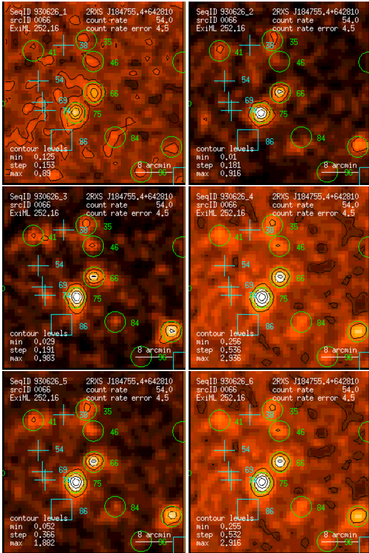
Figure 66: RASS 930626: detection 0066: band rate images, Gaussian filter: (1) PSPC channels 11 – 41, (2) 52 – 90, (3) 91 – 201, (4) 11 – 235, (5) 52 – 201, (6) 11 – 201. Broad band rates in counts/ks. Band rate contour levels in counts/ks/arcmin 2 .
