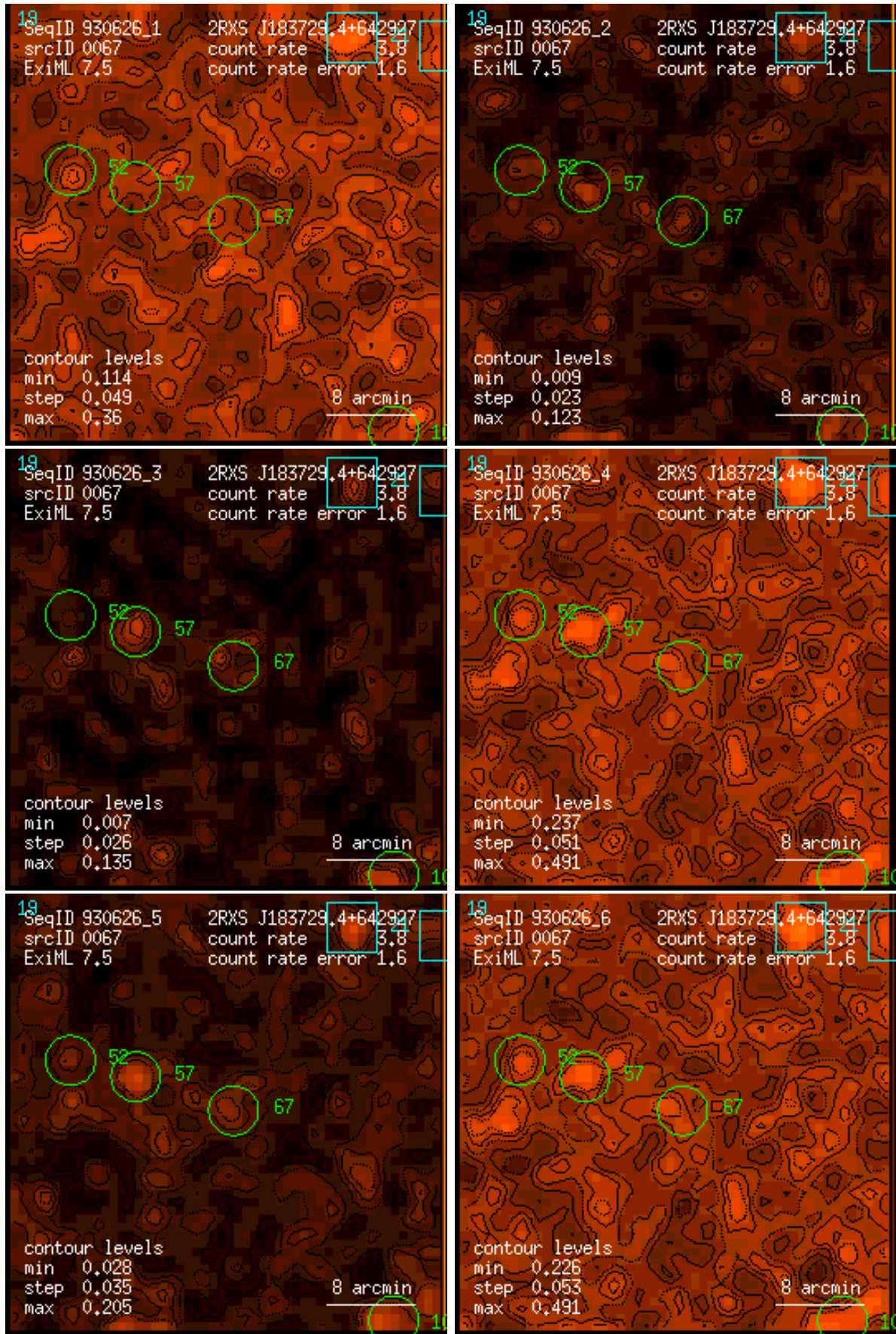
Figure 67: RASS 930626: detection 0067: band rate images, Gaussian filter: (1) PSPC channels 11 – 41, (2) 52 – 90, (3) 91 – 201, (4) 11 – 235, (5) 52 – 201, (6) 11 – 201. Broad band rates in counts/ks. Band rate contour levels in counts/ks/arcmin 2 .
