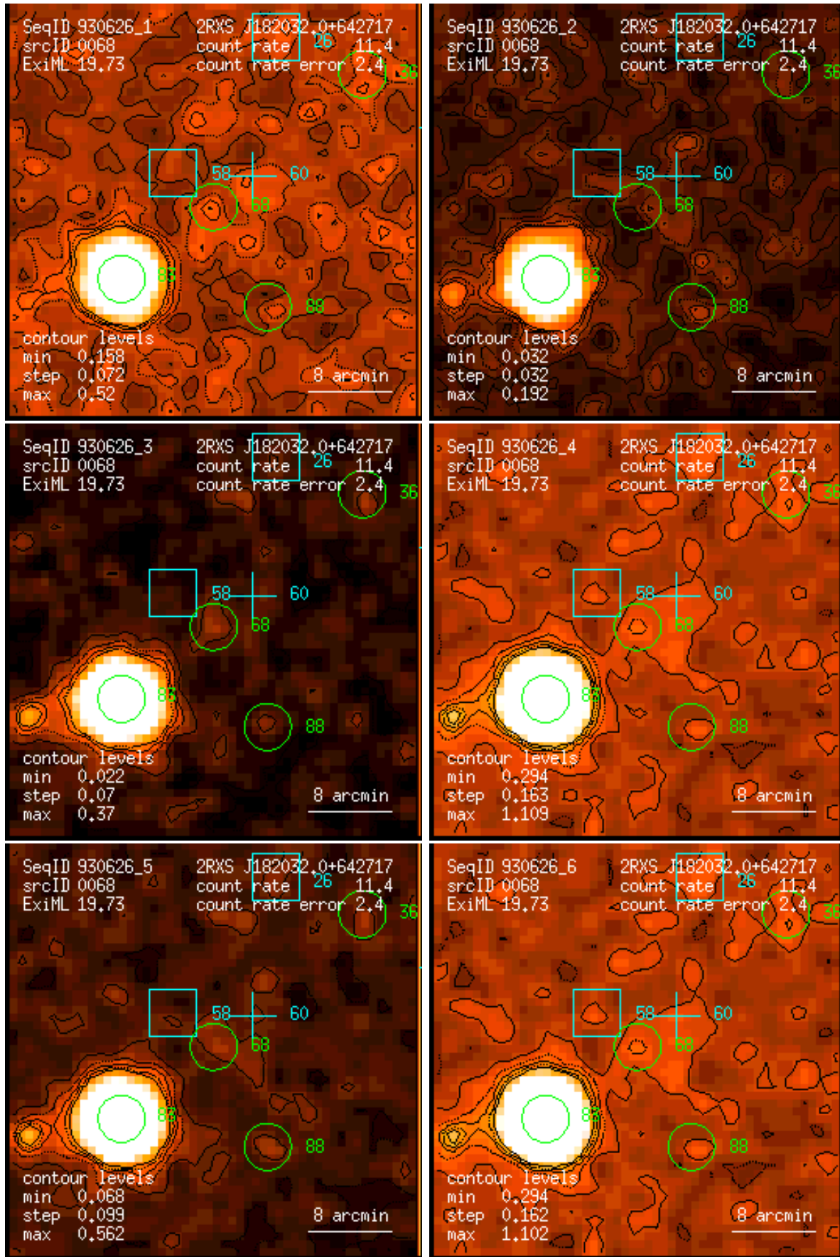
Figure 68: RASS 930626: detection 0068: band rate images, Gaussian filter: (1) PSPC channels 11 – 41, (2) 52 – 90, (3) 91 – 201, (4) 11 – 235, (5) 52 – 201, (6) 11 – 201. Broad band rates in counts/ks. Band rate contour levels in counts/ks/arcmin 2 .
