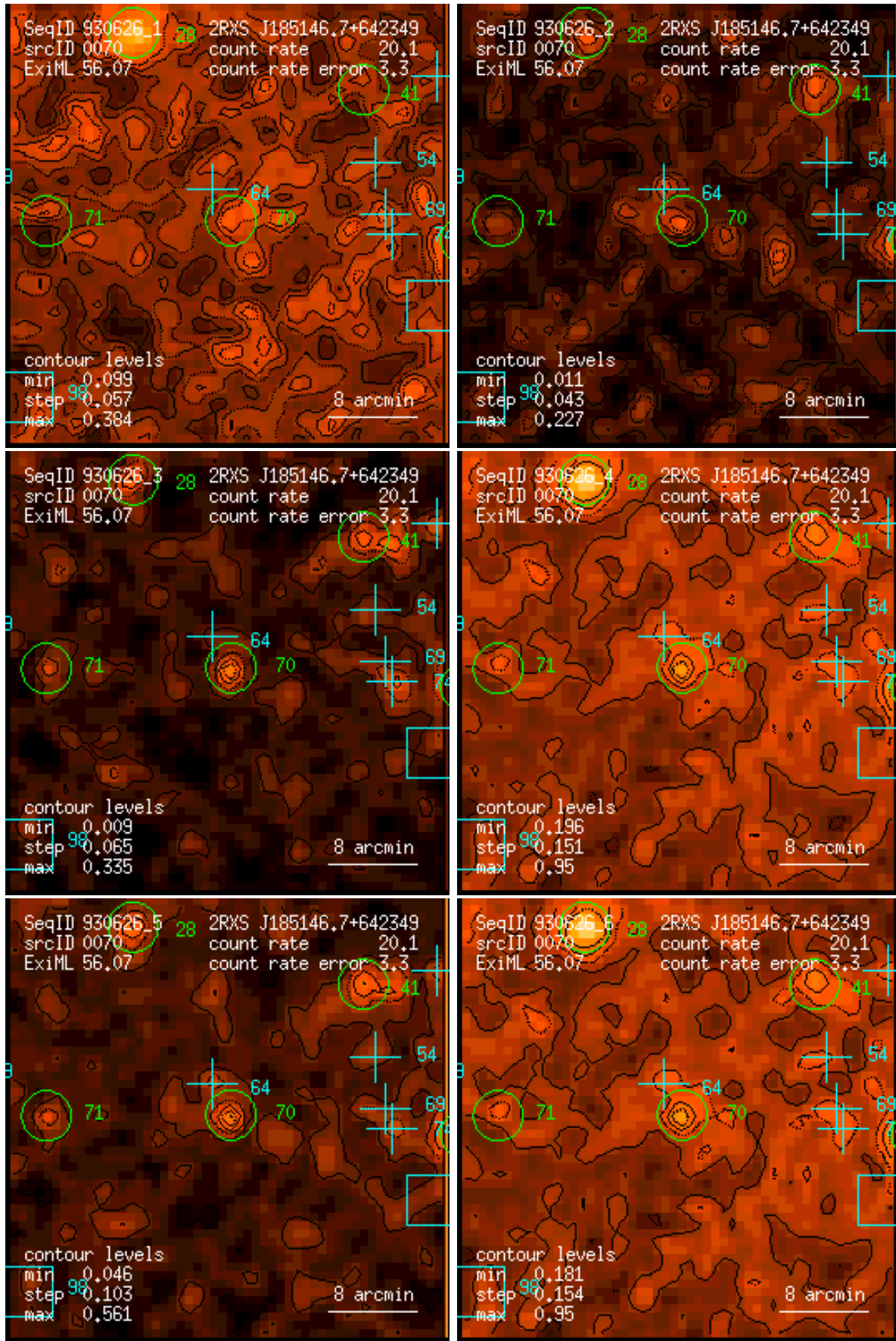
Figure 70: RASS 930626: detection 0070: band rate images, Gaussian filter: (1) PSPC channels 11 – 41, (2) 52 – 90, (3) 91 – 201, (4) 11 – 235, (5) 52 – 201, (6) 11 – 201. Broad band rates in counts/ks. Band rate contour levels in counts/ks/arcmin 2 .
