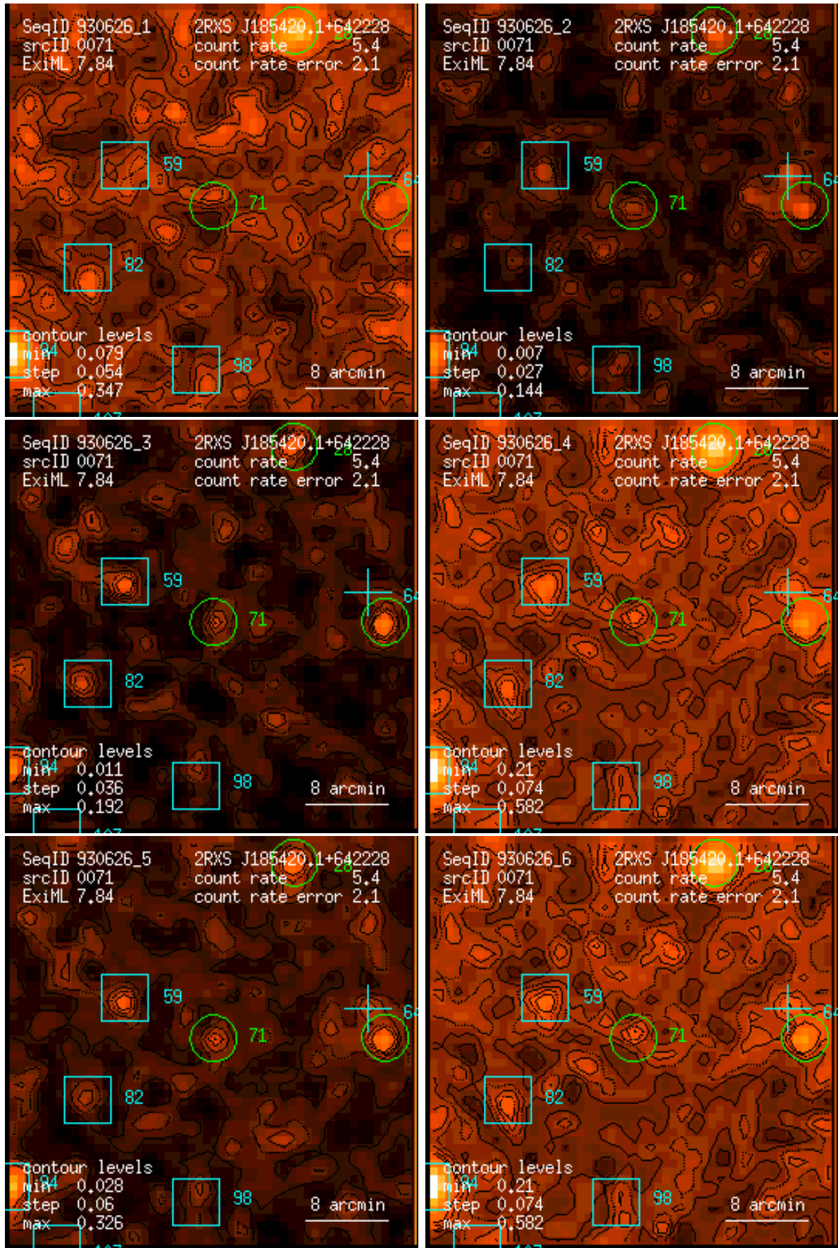
Figure 71: RASS 930626: detection 0071: band rate images, Gaussian filter: (1) PSPC channels 11 – 41, (2) 52 – 90, (3) 91 – 201, (4) 11 – 235, (5) 52 – 201, (6) 11 – 201. Broad band rates in counts/ks. Band rate contour levels in counts/ks/arcmin 2 .
