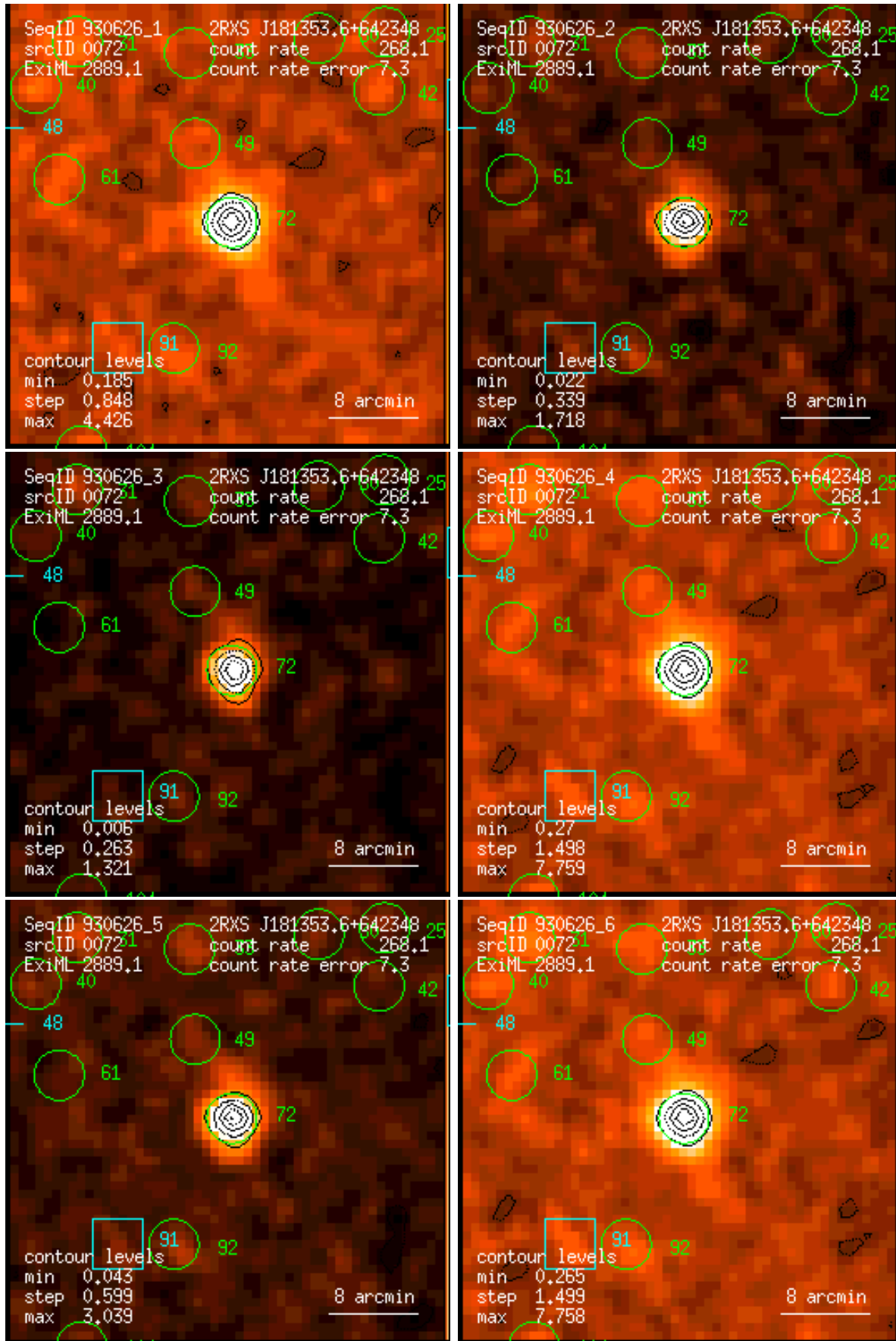
Figure 72: RASS 930626: detection 0072: band rate images, Gaussian filter: (1) PSPC channels 11 – 41, (2) 52 – 90, (3) 91 – 201, (4) 11 – 235, (5) 52 – 201, (6) 11 – 201. Broad band rates in counts/ks. Band rate contour levels in counts/ks/arcmin 2 .
