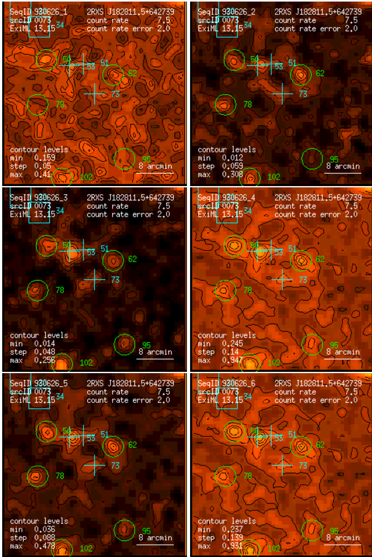
Figure 73: RASS 930626: detection 0073: band rate images, Gaussian filter: (1) PSPC channels 11 – 41, (2) 52 – 90, (3) 91 – 201, (4) 11 – 235, (5) 52 – 201, (6) 11 – 201. Broad band rates in counts/ks. Band rate contour levels in counts/ks/arcmin 2 .
