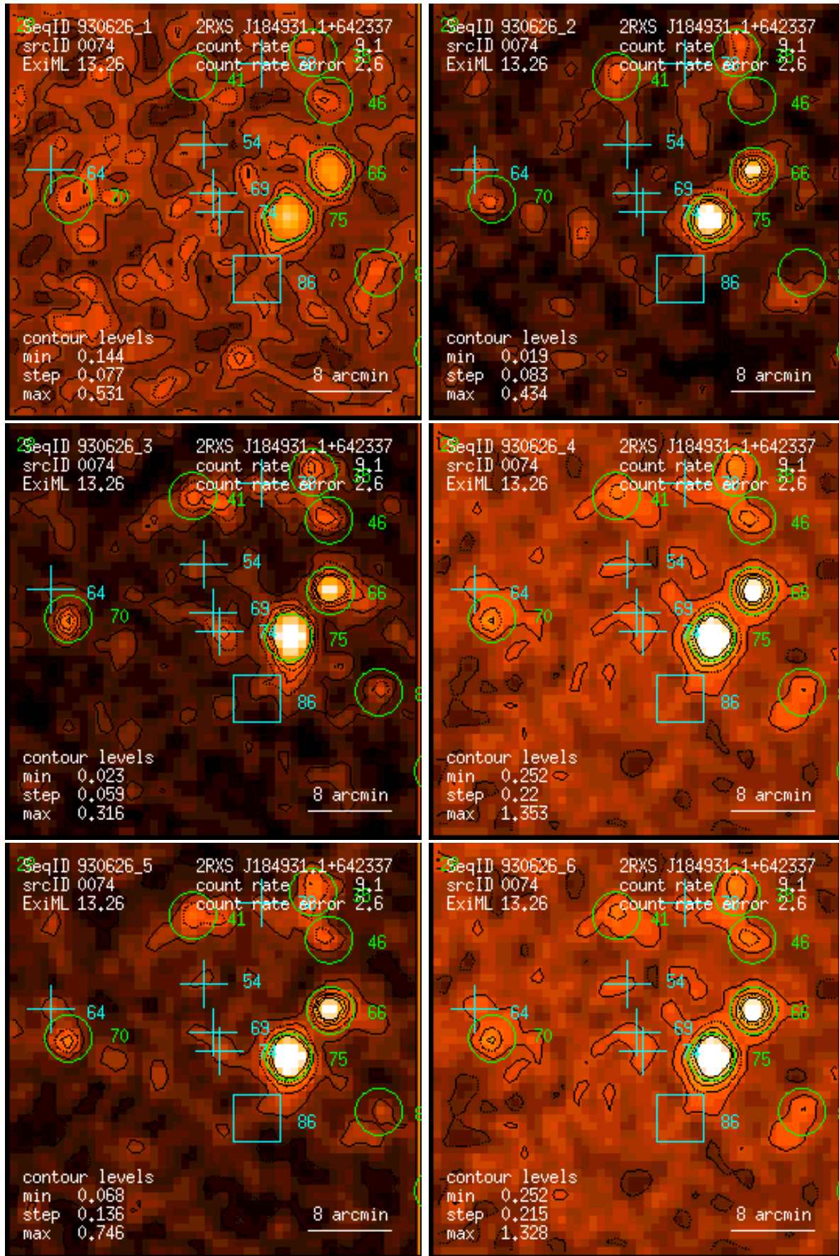
Figure 74: RASS 930626: detection 0074: band rate images, Gaussian filter: (1) PSPC channels 11 – 41, (2) 52 – 90, (3) 91 – 201, (4) 11 – 235, (5) 52 – 201, (6) 11 – 201. Broad band rates in counts/ks. Band rate contour levels in counts/ks/arcmin 2 .
