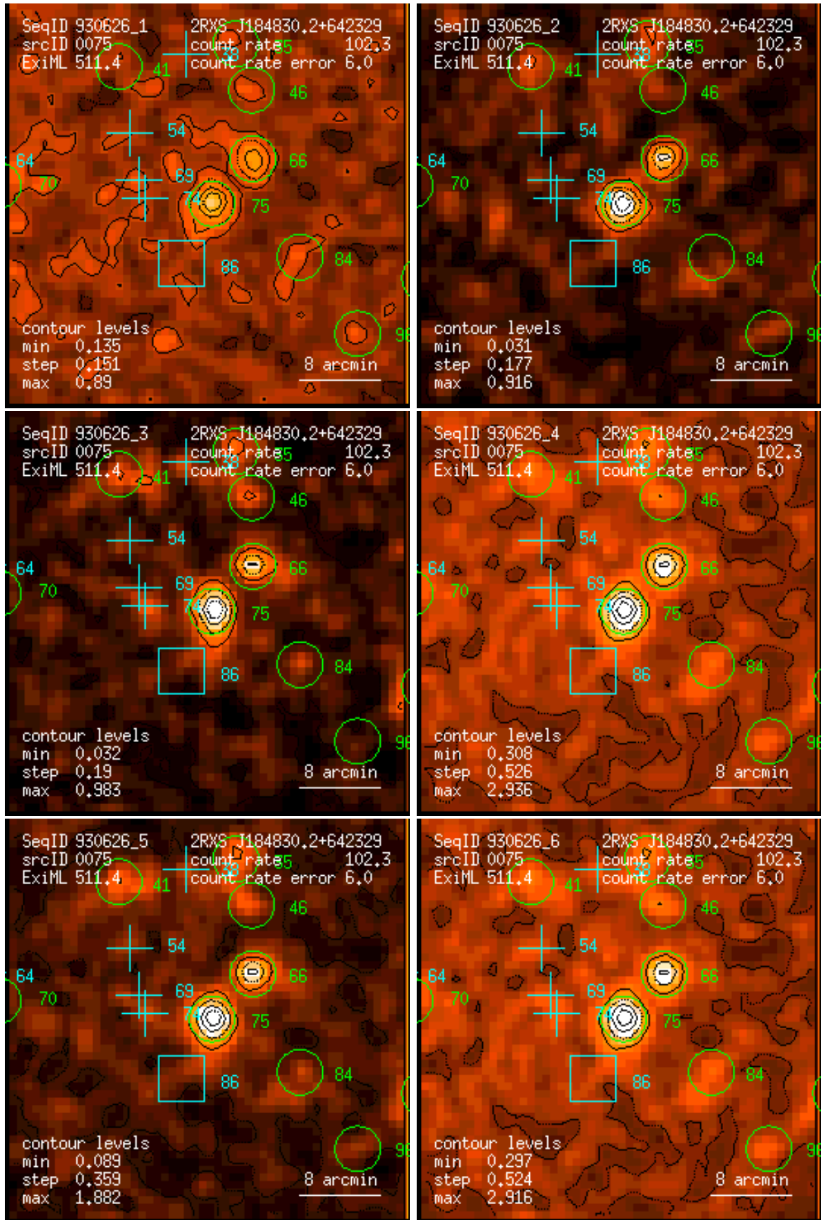
Figure 75: RASS 930626: detection 0075: band rate images, Gaussian filter: (1) PSPC channels 11 – 41, (2) 52 – 90, (3) 91 – 201, (4) 11 – 235, (5) 52 – 201, (6) 11 – 201. Broad band rates in counts/ks. Band rate contour levels in counts/ks/arcmin 2 .
