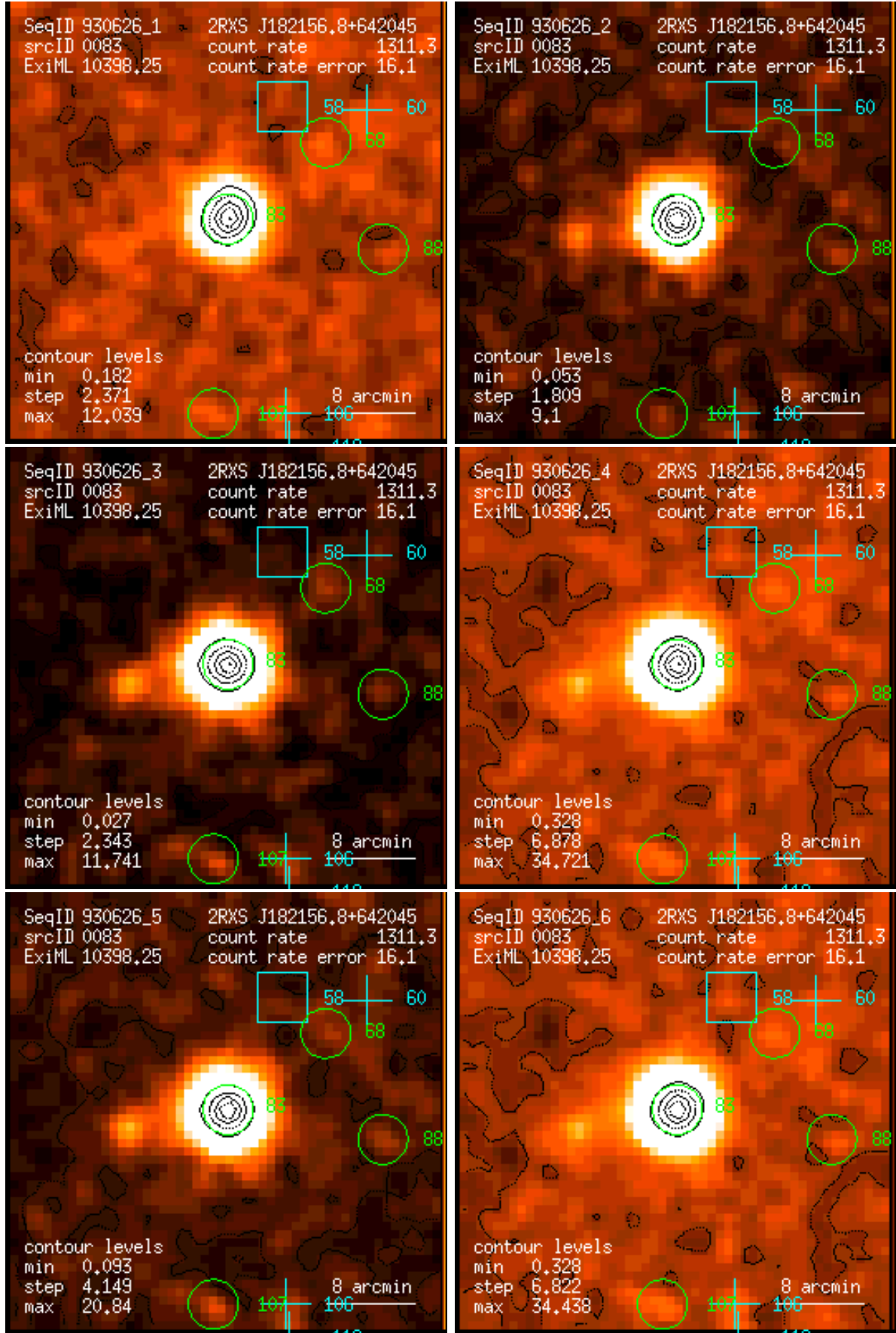
Figure 83: RASS 930626: detection 0083: band rate images, Gaussian filter: (1) PSPC channels 11 – 41, (2) 52 – 90, (3) 91 – 201, (4) 11 – 235, (5) 52 – 201, (6) 11 – 201. Broad band rates in counts/ks. Band rate contour levels in counts/ks/arcmin 2 .
