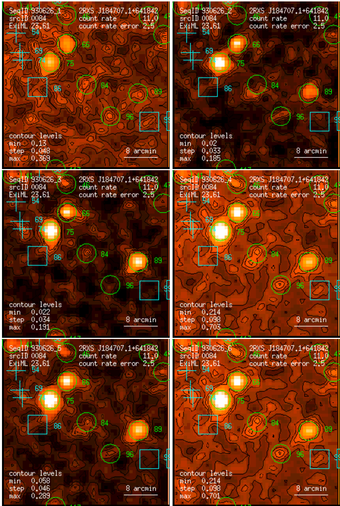
Figure 84: RASS 930626: detection 0084: band rate images, Gaussian filter: (1) PSPC channels 11 – 41, (2) 52 – 90, (3) 91 – 201, (4) 11 – 235, (5) 52 – 201, (6) 11 – 201. Broad band rates in counts/ks. Band rate contour levels in counts/ks/arcmin 2 .
