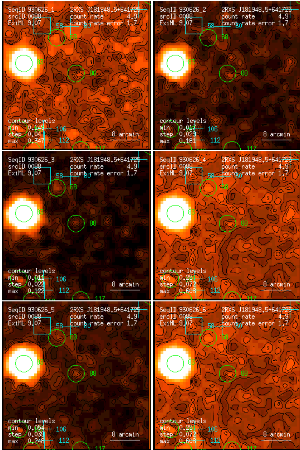
Figure 88: RASS 930626: detection 0088: band rate images, Gaussian filter: (1) PSPC channels 11 – 41, (2) 52 – 90, (3) 91 – 201, (4) 11 – 235, (5) 52 – 201, (6) 11 – 201. Broad band rates in counts/ks. Band rate contour levels in counts/ks/arcmin 2 .
