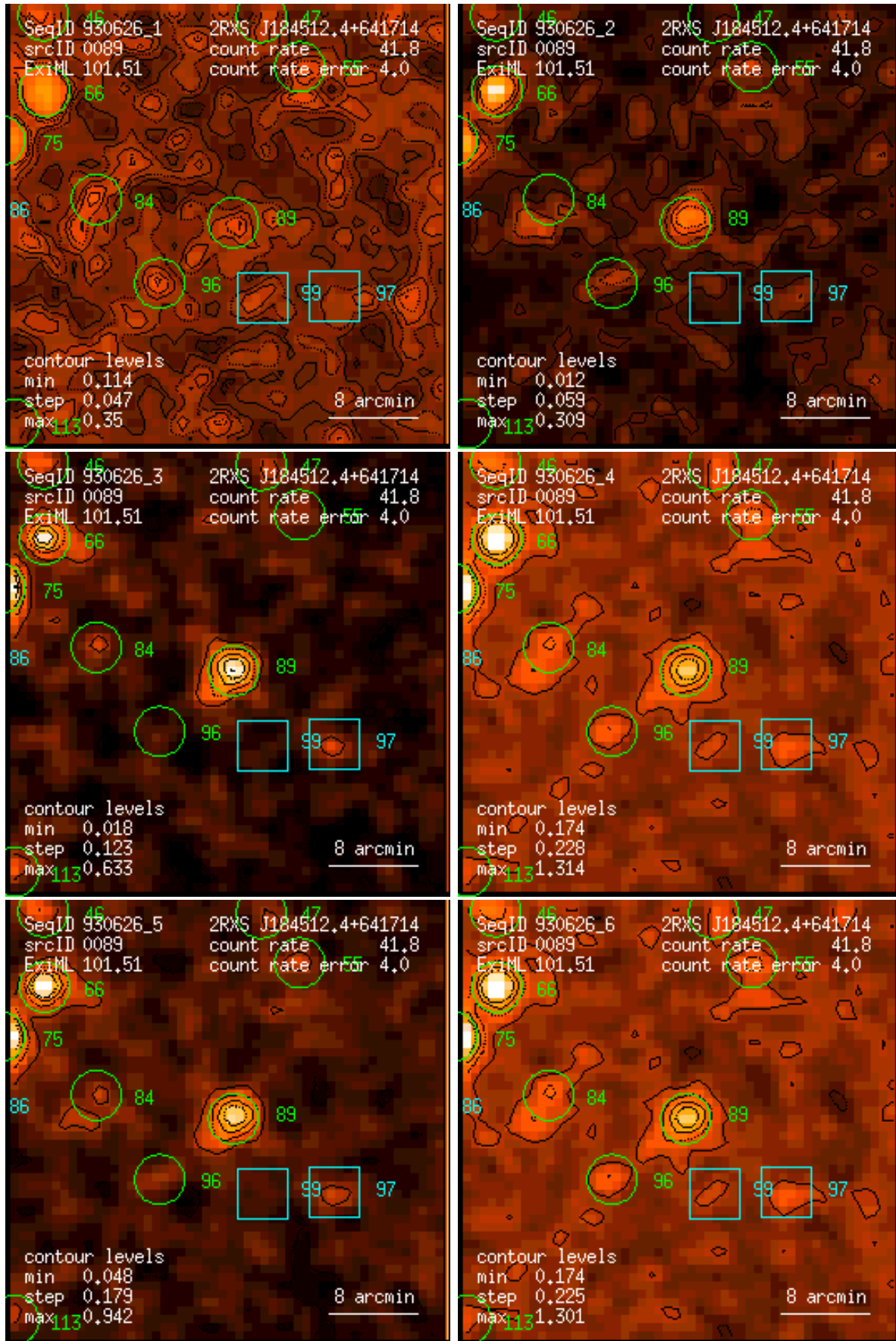
Figure 89: RASS 930626: detection 0089: band rate images, Gaussian filter: (1) PSPC channels 11 – 41, (2) 52 – 90, (3) 91 – 201, (4) 11 – 235, (5) 52 – 201, (6) 11 – 201. Broad band rates in counts/ks. Band rate contour levels in counts/ks/arcmin 2 .
