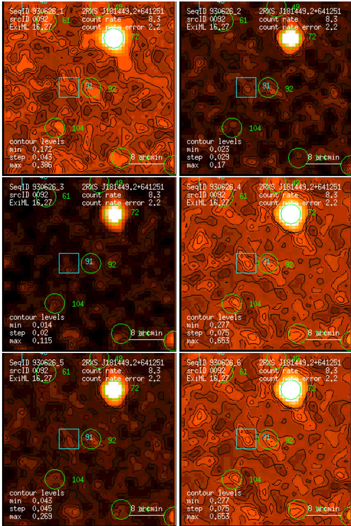
Figure 92: RASS 930626: detection 0092: band rate images, Gaussian filter: (1) PSPC channels 11 – 41, (2) 52 – 90, (3) 91 – 201, (4) 11 – 235, (5) 52 – 201, (6) 11 – 201. Broad band rates in counts/ks. Band rate contour levels in counts/ks/arcmin 2 .
