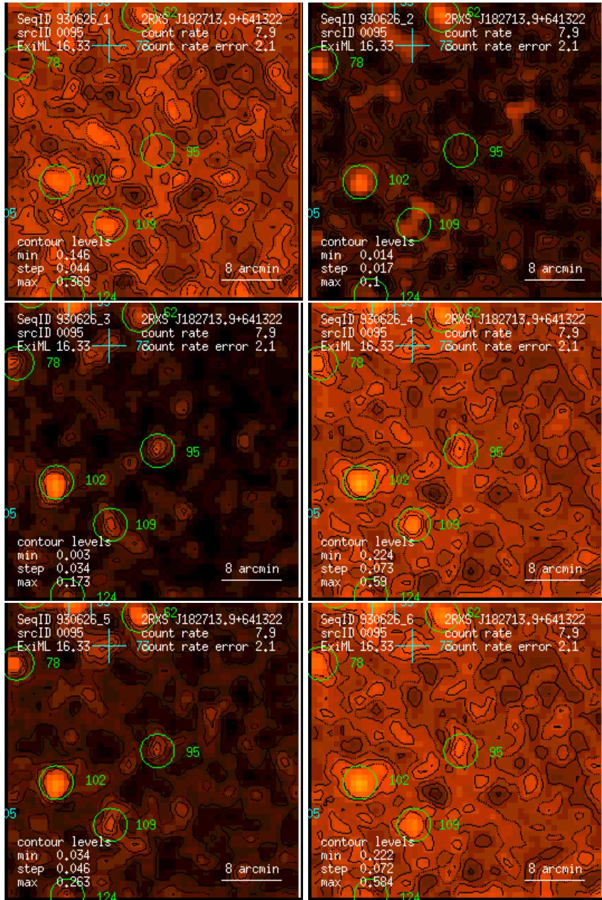
Figure 95: RASS 930626: detection 0095: band rate images, Gaussian filter: (1) PSPC channels 11 – 41, (2) 52 – 90, (3) 91 – 201, (4) 11 – 235, (5) 52 – 201, (6) 11 – 201. Broad band rates in counts/ks. Band rate contour levels in counts/ks/arcmin 2 .
