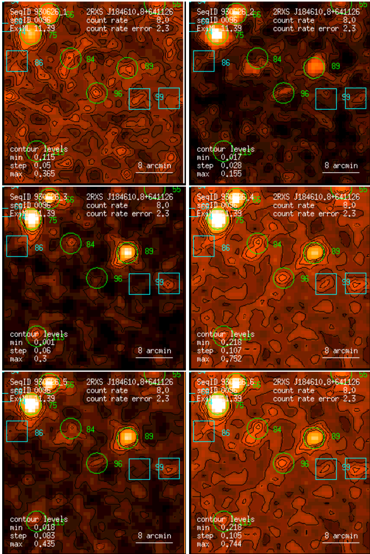
Figure 96: RASS 930626: detection 0096: band rate images, Gaussian filter: (1) PSPC channels 11 – 41, (2) 52 – 90, (3) 91 – 201, (4) 11 – 235, (5) 52 – 201, (6) 11 – 201. Broad band rates in counts/ks. Band rate contour levels in counts/ks/arcmin 2 .
