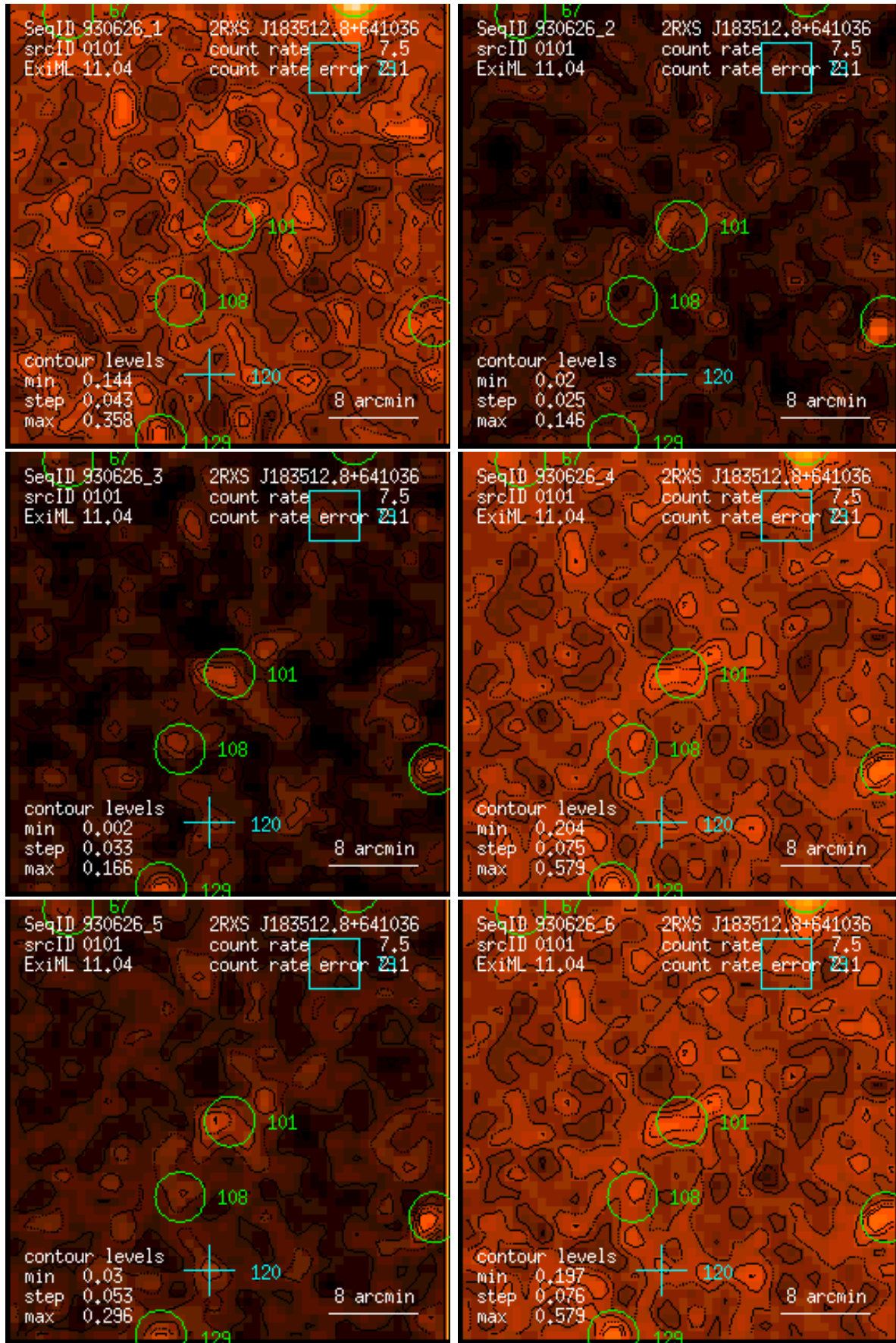
Figure 101: RASS 930626: detection 0101: band rate images, Gaussian filter: (1) PSPC channels 11 – 41, (2) 52 – 90, (3) 91 – 201, (4) 11 – 235, (5) 52 – 201, (6) 11 – 201. Broad band rates in counts/ks. Band rate contour levels in counts/ks/arcmin 2 .
