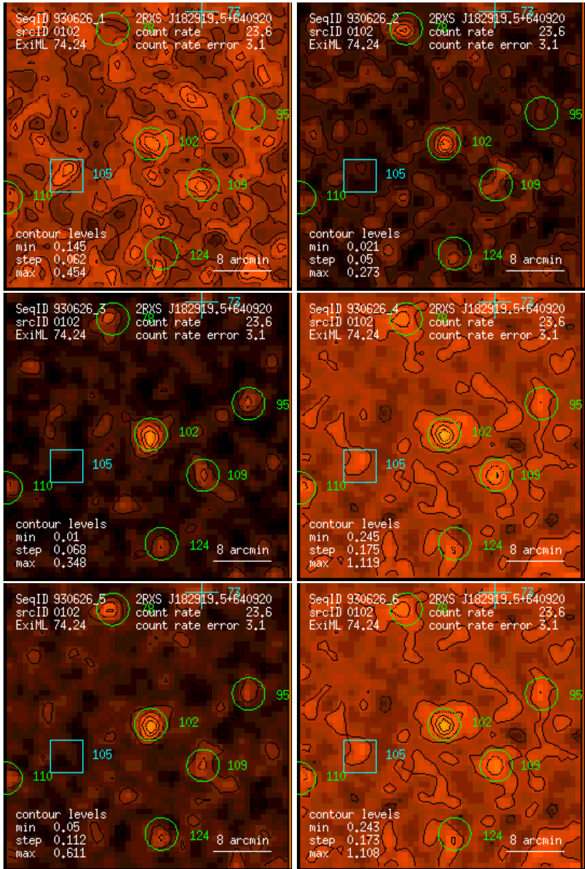
Figure 102: RASS 930626: detection 0102: band rate images, Gaussian filter: (1) PSPC channels 11 – 41, (2) 52 – 90, (3) 91 – 201, (4) 11 – 235, (5) 52 – 201, (6) 11 – 201. Broad band rates in counts/ks. Band rate contour levels in counts/ks/arcmin 2 .
