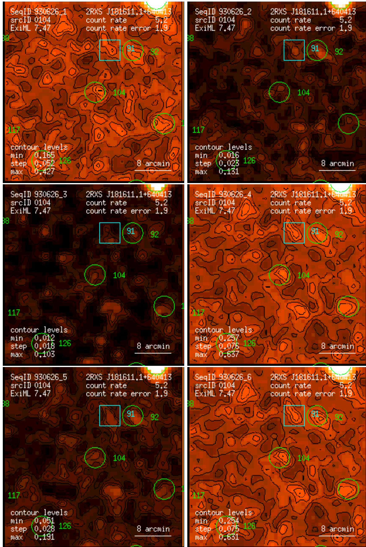
Figure 104: RASS 930626: detection 0104: band rate images, Gaussian filter: (1) PSPC channels 11 – 41, (2) 52 – 90, (3) 91 – 201, (4) 11 – 235, (5) 52 – 201, (6) 11 – 201. Broad band rates in counts/ks. Band rate contour levels in counts/ks/arcmin 2 .
