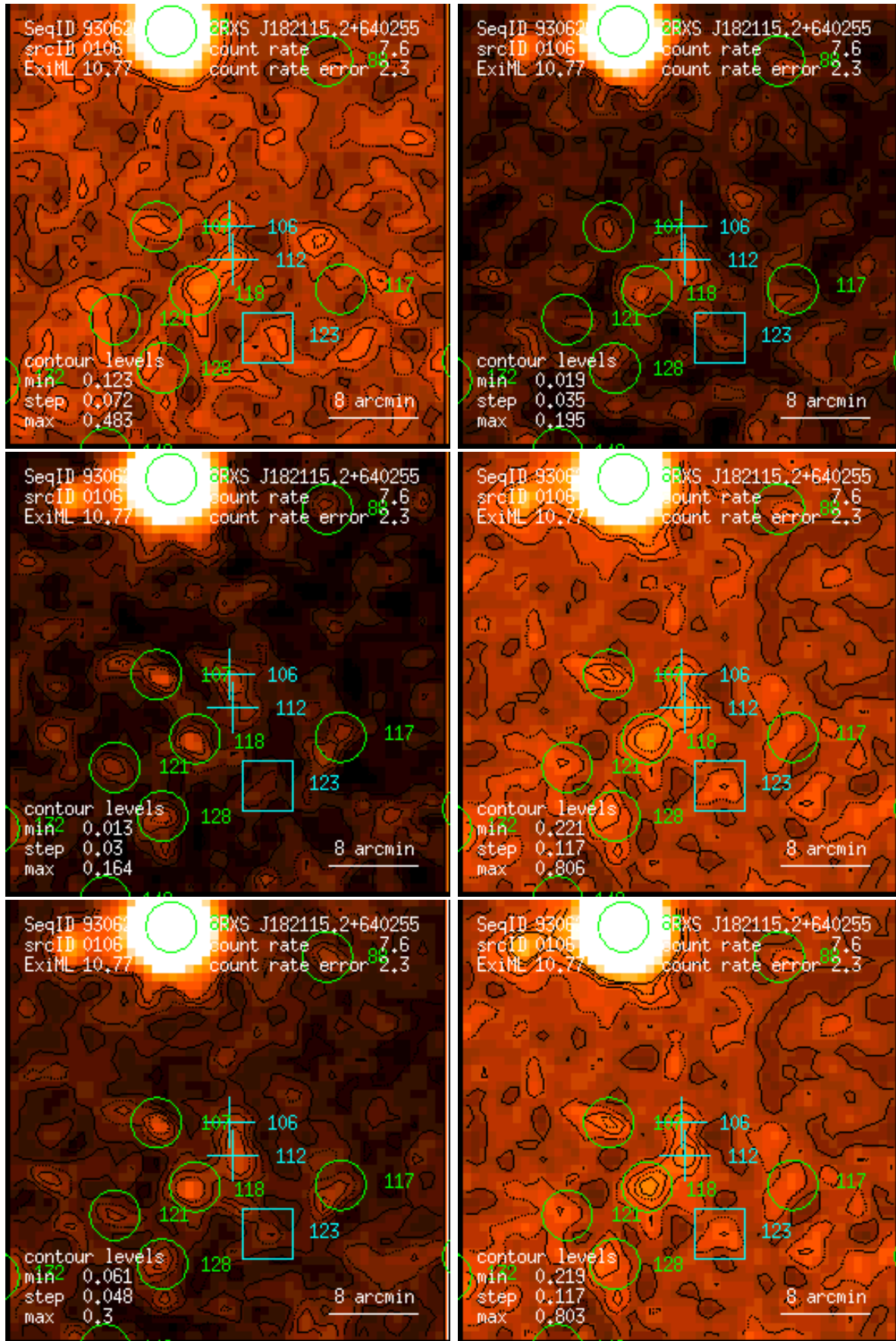
Figure 106: RASS 930626: detection 0106: band rate images, Gaussian filter: (1) PSPC channels 11 – 41, (2) 52 – 90, (3) 91 – 201, (4) 11 – 235, (5) 52 – 201, (6) 11 – 201. Broad band rates in counts/ks. Band rate contour levels in counts/ks/arcmin 2 .
