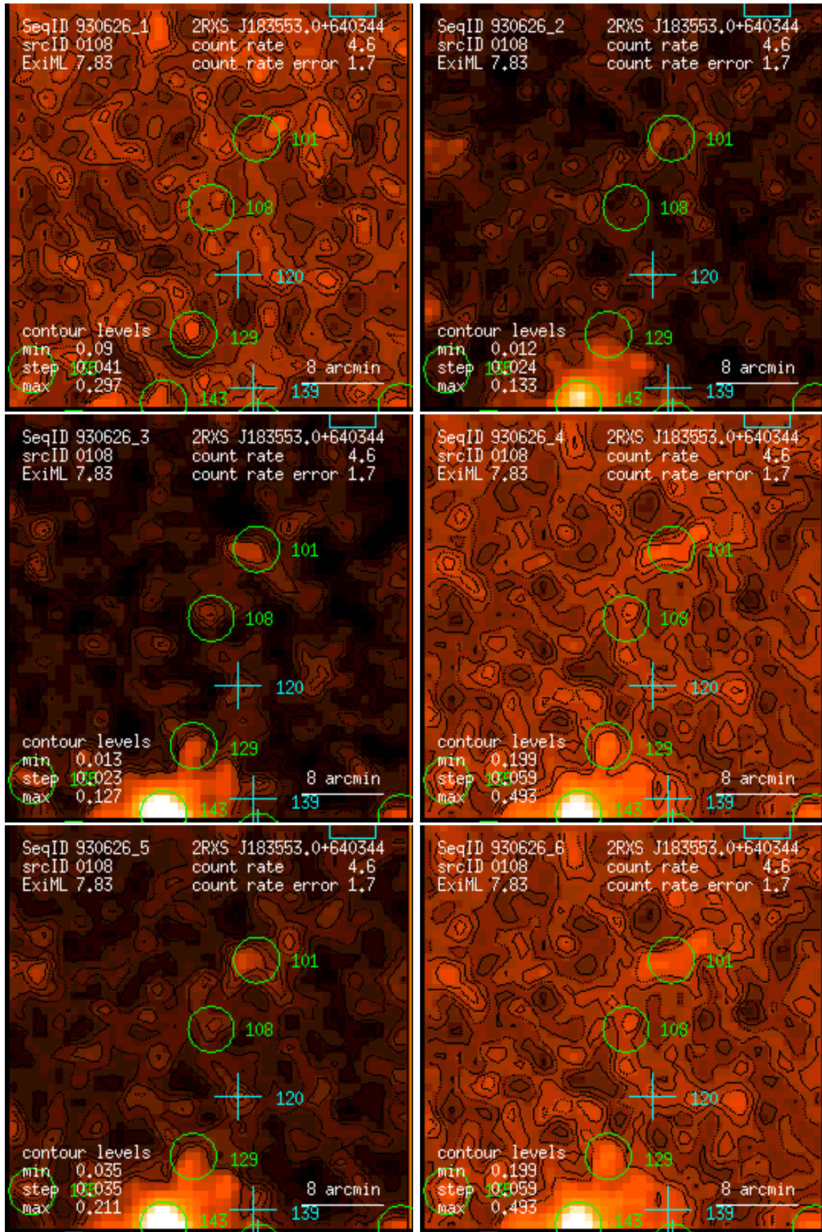
Figure 108: RASS 930626: detection 0108: band rate images, Gaussian filter: (1) PSPC channels 11 – 41, (2) 52 – 90, (3) 91 – 201, (4) 11 – 235, (5) 52 – 201, (6) 11 – 201. Broad band rates in counts/ks. Band rate contour levels in counts/ks/arcmin 2 .
